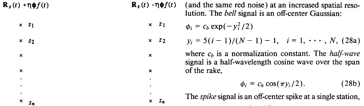
FIG. 4. The model coupled system (explained in the text).
