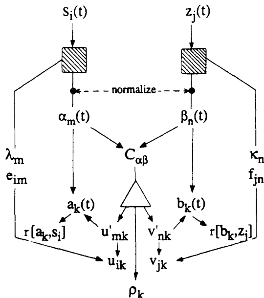
FIG. 2. As in Fig. 1 except for CCA. The squares represent PCA operations. PCA and SVD symbols are darkened for steps in which only a leading subset of the modes in the expansion is retained.
