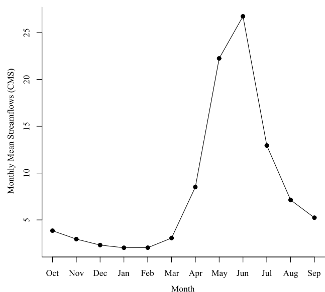
Figure 2. Annual average hydrograph of the Gunnison River Basin. Monthly values (m 3 /s (cms)) are the average across the six locations.
