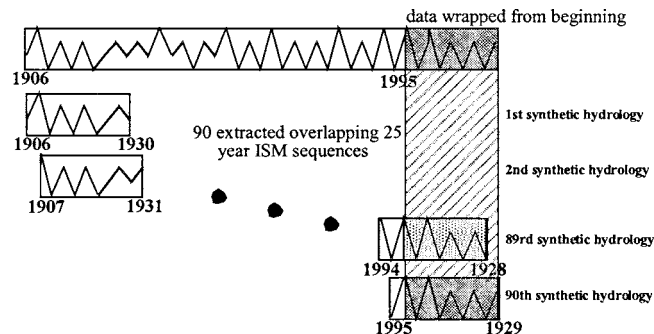
Fig. 1. Schematic of the ISM [adapted from Ouarda et al. (1997)]. The synthetic hydrologies, each 25 years in length, are shown below the original 90-year time series. The additional 24 years used for wraparound are shown in shading.
