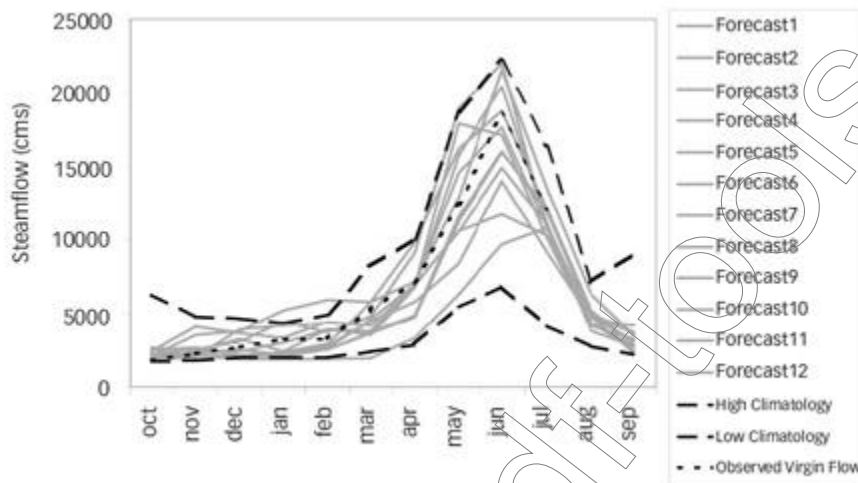
Figure 6.4 Streamflow forecast for the Columbia River for 1999. This graph is based on resampling from the historical record using analog conditions to predicted ENSO and PDO phase, as well as snowpack conditions produced. Produced in June and offering a six month lead-time.
