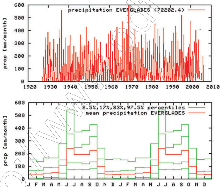
Figure 4.13 Precipitation analyses using the KNMI Climate Explorer. Some investigative data analyses using the KNMI Climate Explorer applied to a specific watershed, the Everglades in the United States. Precipitation shown (a) as raw time series, and (b) by month, with selected probability curves. These graphs can be used to illustrate the historical distribution of precipitation for a given system.
