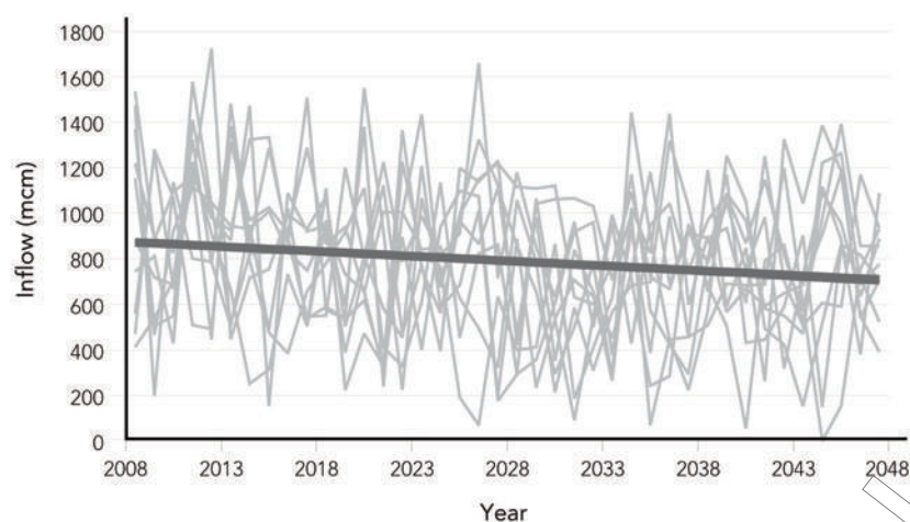
Figure 5.9 (a) Projected inflow traces with a long-term trend of -20%, interannual variability consistent with the historical record, and no systematically imposed multidecadal variability. (Traces sampled from 100 simulations by selecting every 10th trace after ranking by average inflow. Includes trendline average for all inflow traces (4.2mcm/year decrease))
