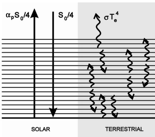
Figure 2.10: Schematic of radiative transfer model with many layers.
