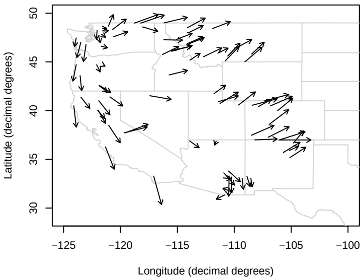
Vector Plot of Streamflow for 1971–2000 (Indiv. F at frequency of 1 cyc/yr)
