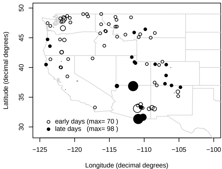
Phase Shift of Streamflow (1940–1970,1971–2000) (Indiv. F at frequency of 1 cyc/yr)
