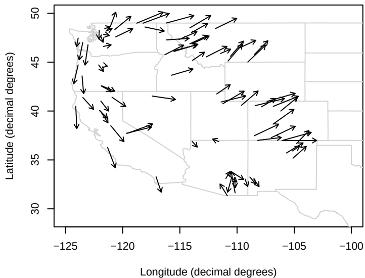
Vector Plot of Streamflow for 1940–1970 (Indiv. F at frequency of 1 cyc/yr)
