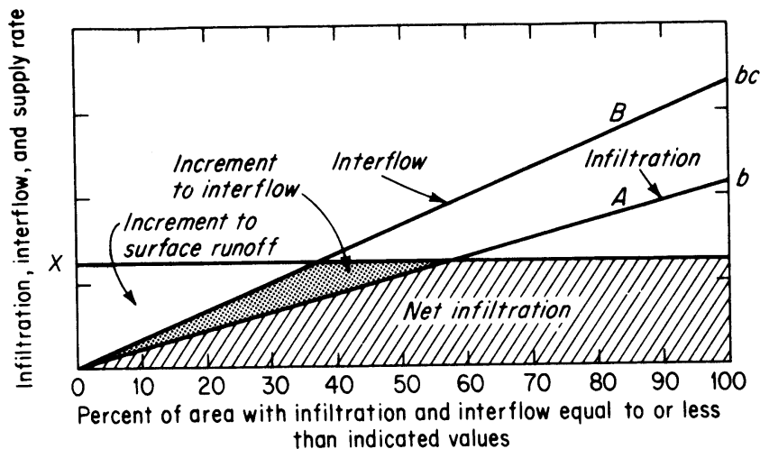
Figure 54. Infiltration-interflow function used in the Sacramento Model (from Linsley et al., 1982).
