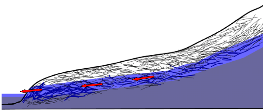
Figure 10. Schematic illustration of macropore network being activated due to rise in groundwater resulting in rapid lateral flow.
