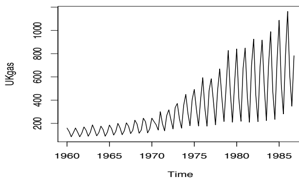
Fig. 2.2. Quarterly UK gas consumption from 1960Q1 to 1986Q4, in millions of therms.
