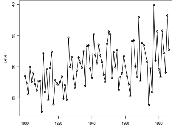
Fig. 3.2. Annual precipitation at Lake Superior
