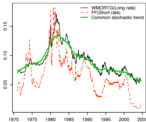
Fig. 5.5. Posterior mean of the common stochastic trend
