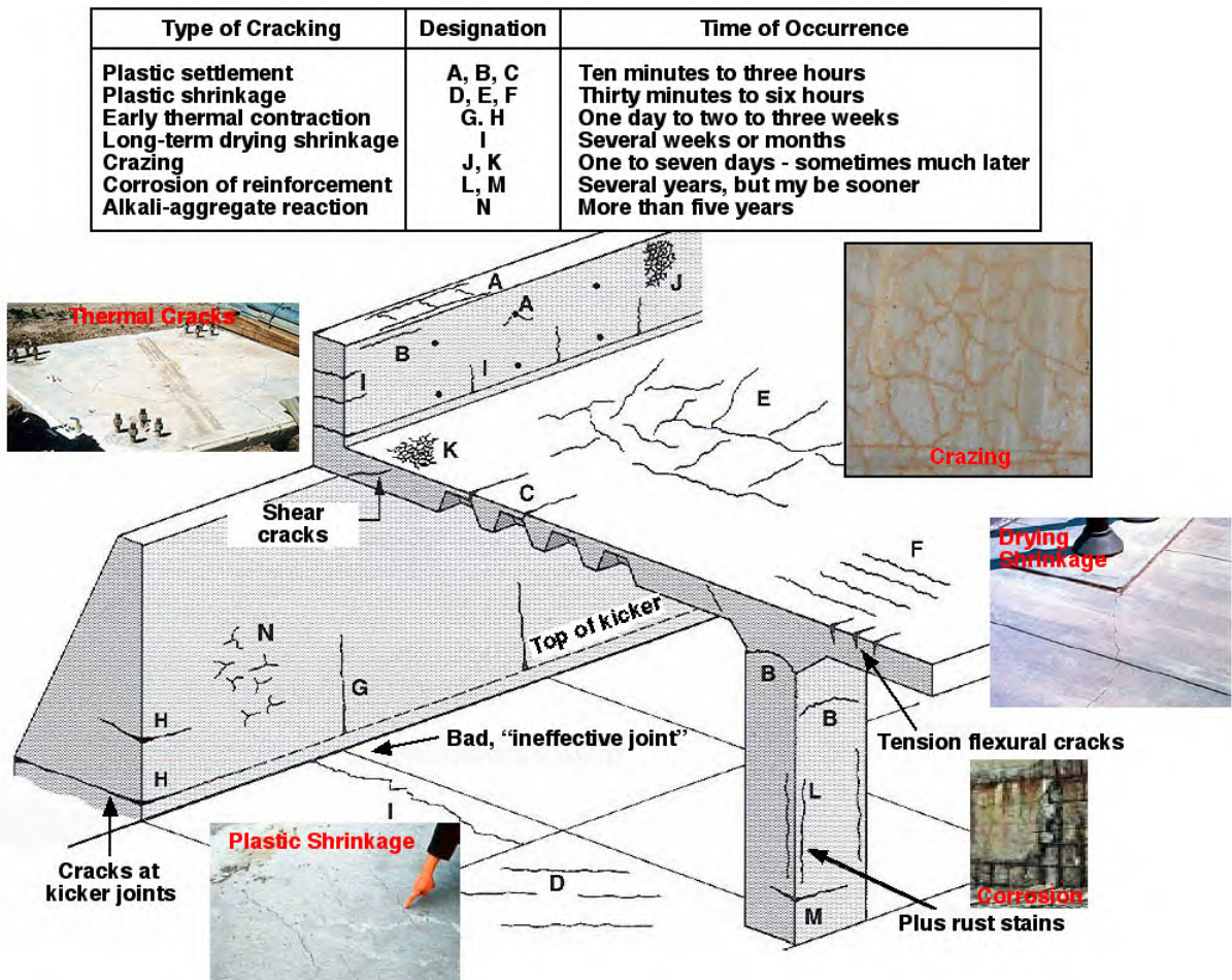
Figure 4.1. Examples of intrinsic cracks in a hypothetical structure [42].
