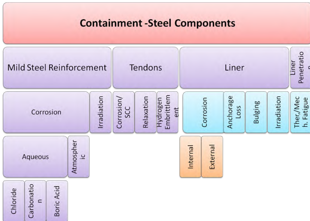
Figure 1.2. Degradation modes in reactor containments: steel components.
