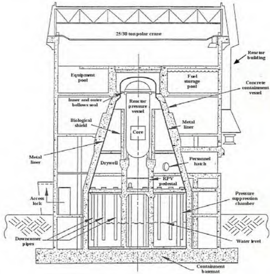
Figure 2.2. BWR Mark II type reinforced concrete containment [13].
