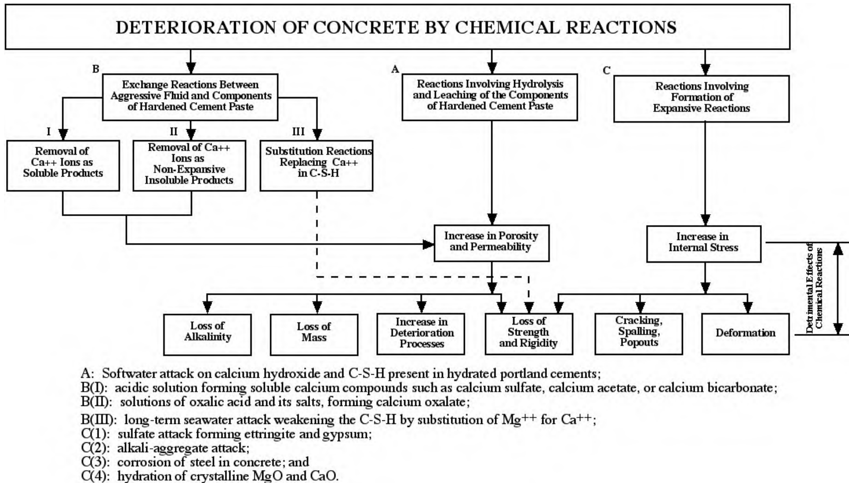
Figure 4.5. Types of chemical reactions responsible for concrete deterioration [80].
