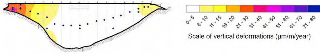
Figure 3.97: Vertical swelling rates observed on dam n-18; Guilloteau, Martinot, and Sausse (2017)
