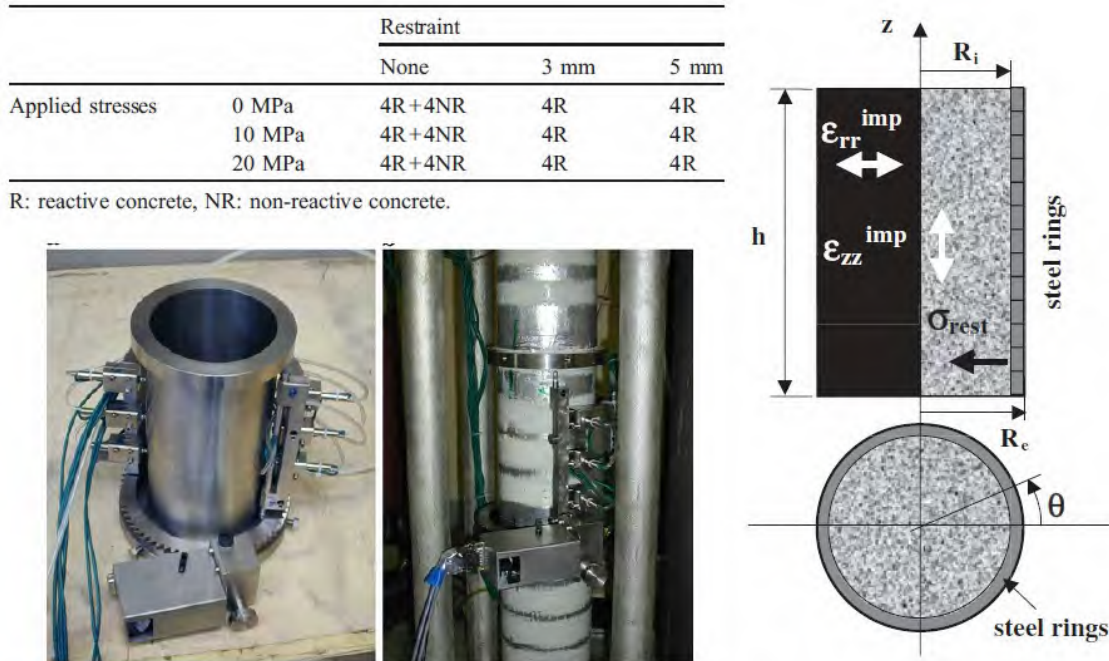
Figure 3.156: Characteristics of the 48 specimens including the steel rings and strain measurements by an automated device; Multon and Toutlemonde (2006)
