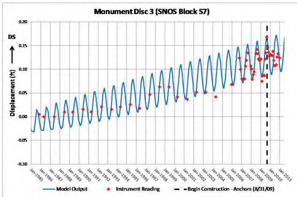
Figure 178. Monument Disc 3 Instrument Reading vs. Model Output (2013)
