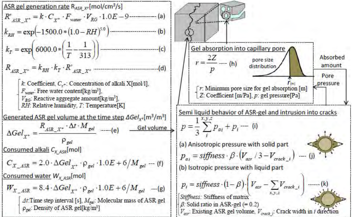
Figure 3.96: Calculation scheme for ASR gel generation and stress formation
