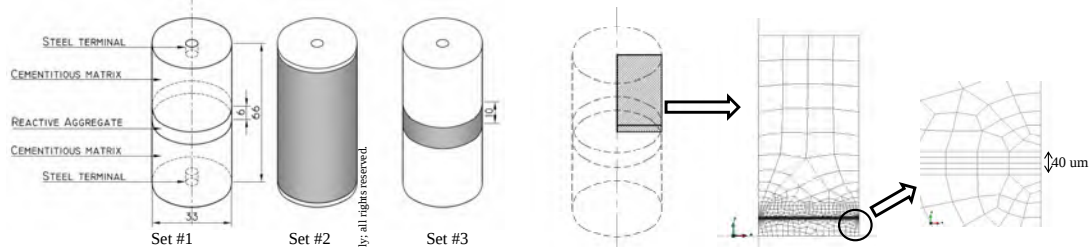
Figure 5. Model geometry and FE mesh.
