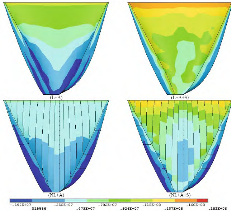
Figure 3.133: Contours of the 1st principal stresses on downstream face for the time of 1800 days (L: Linear; A: AAR; NL: Joint); Lamea and Mirzabozorg (2015)
