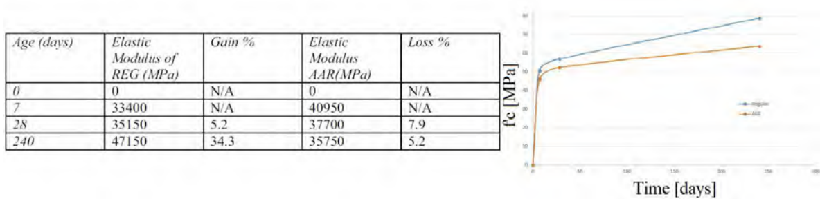
Figure 3.164: ASR effects on material tests; Orbovic et al. (2015)
