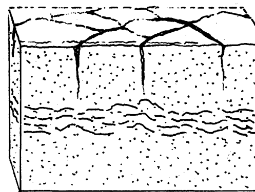
Fig. 9. Effect of compressive stress on expansion due to AAR (from ISE 1992).
