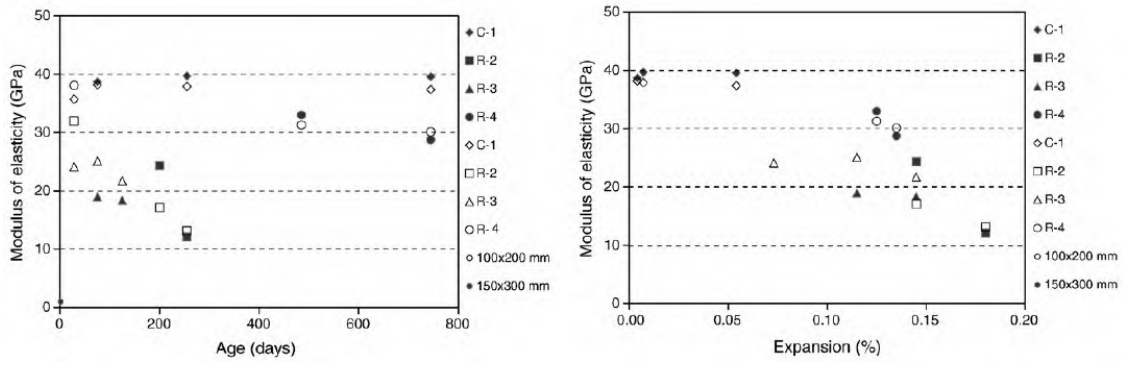
Figure 3.88: Variation of modulus of elasticity with age and expansion; Giaccio et al. (2008)
