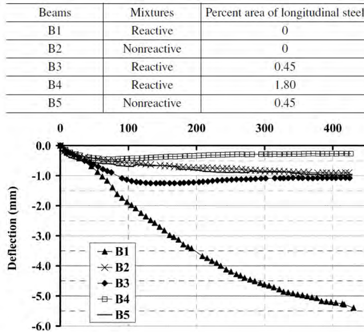
Figure 3.155: Mean deflection of five beams at midspan; Multon, Seignol, and Toutlemonde (2005)
