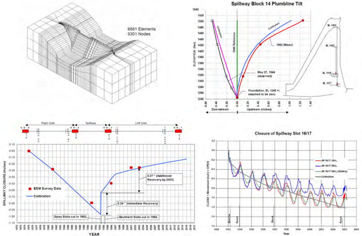
Figure 3.42: FE model and calibration results; Curtis et al. (2005)
