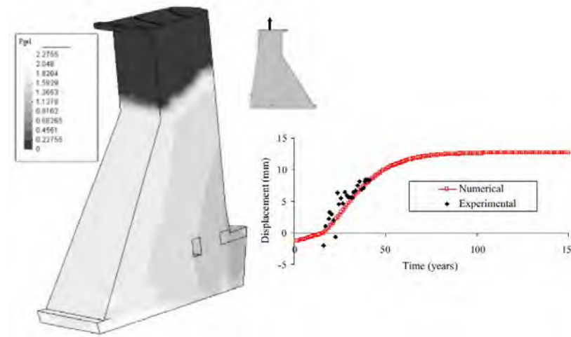
Figure 3.66: Results for the ASR simulation: gel pressure for 40 years and the displacements at the crest of the dam; Fairbairn et al. (2006)
