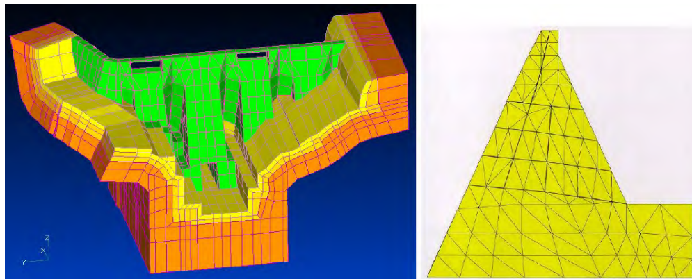
Figure 3.54: Finite element model; Donghi, Marcello, and Sainati (2013)
