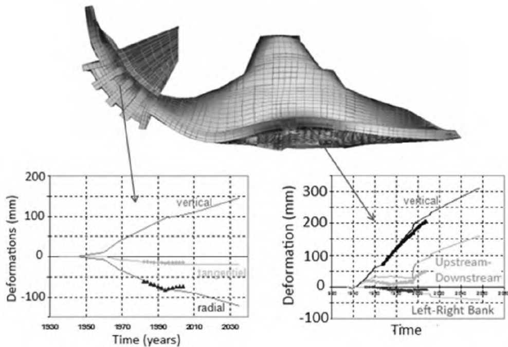
Figure 3.153: Comparison of measured and computed deformations in 3D; Morenon et al. (2018)
