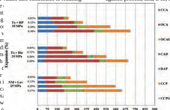
(a) 25 MPa mixtures
