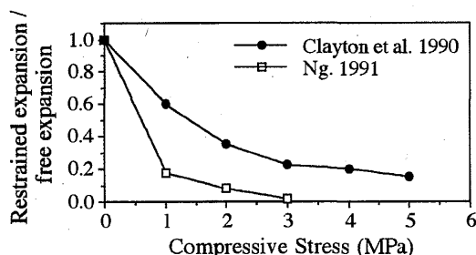
Fig. 9. Effect of compressive stress on expansion due to AAR (from ISE 1992).
