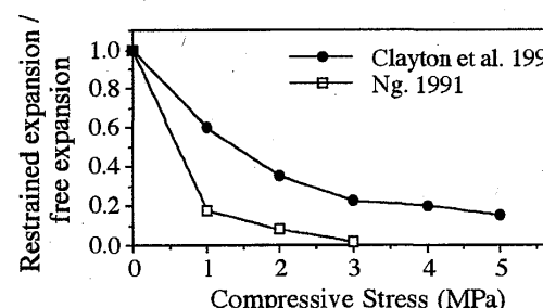
Fig. 9. Effect of compressive stress on expansion due to AAR (from ISE 1992).
