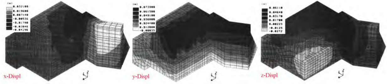
Figure 3.115: Contours of displacement components after 25 years of the reaction; Huang and Pietruszczak (1996)
