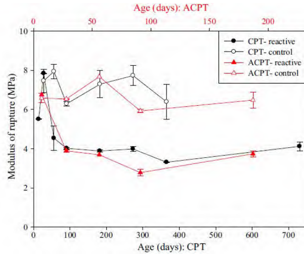
Figure 3.84: Variation in modulus of rupture of concrete prism specimens over time using different time scales; Gautam and Panesar (2017)
