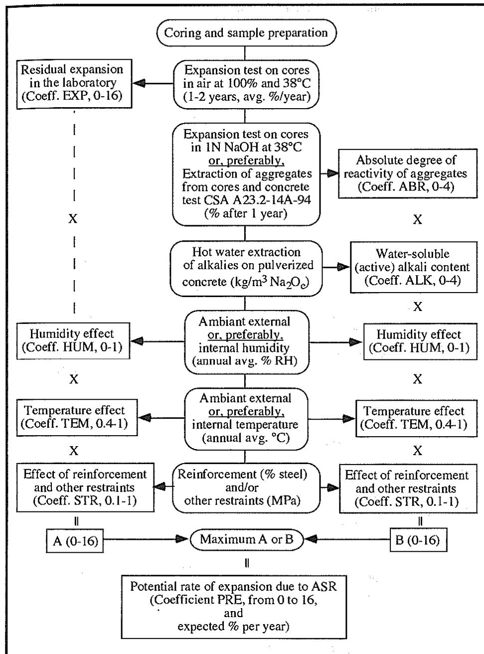
Fig. 1: Laboratory assessment of the potential rate of ASR expansion of concrete members in service either already affected by ASR or not. Figure 3.16: Laboratory assessment of the potential rate of ASR expansion members in service either already affected by ASR or not
