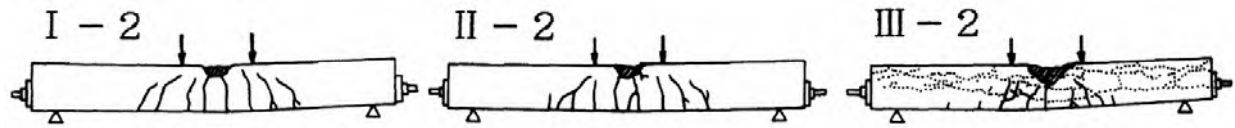
Figure 3.131: Failure modes; Kobayashi et al. (1988)
