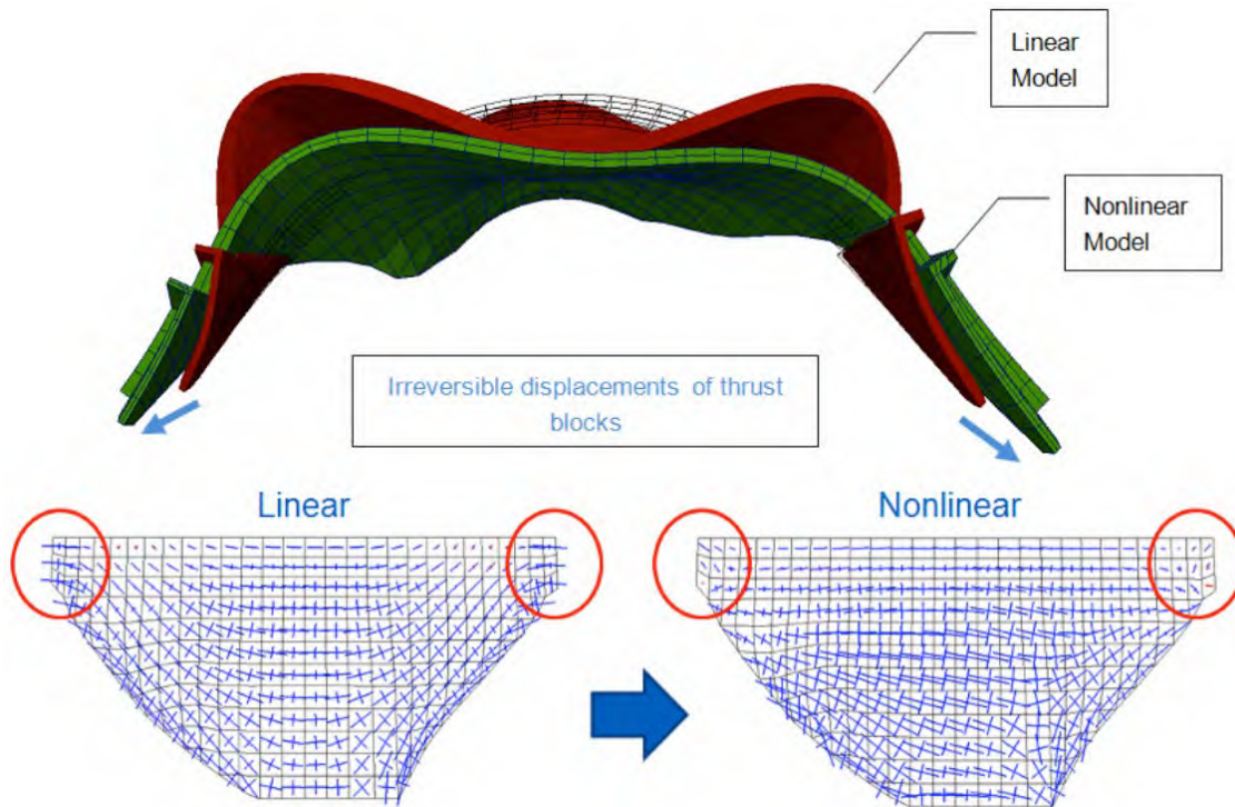
Figure 3.35: Linear model and nonlinear model with concrete-to-rock joint on a swelling arch dam with thrust blocks; Stress reorientation and modification on the upstream face; Coubard and Sausse (2017)
