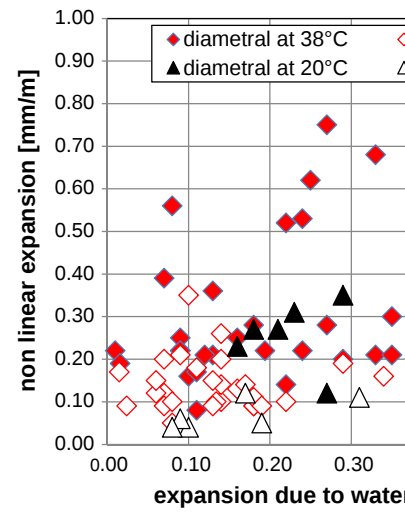
Fig. 4. Non-linear expansion at the beginning of water adsorption during conditioning of the samples.
