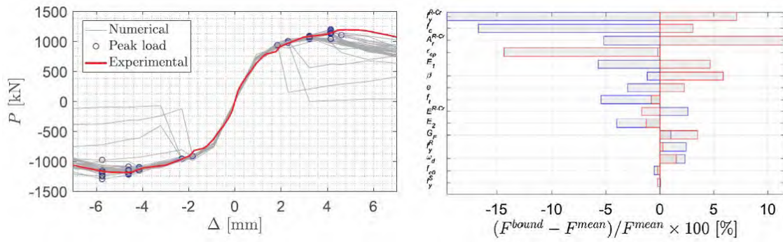
Figure 3.107: Results of sensitivity analysis on concrete constitutive model, capacity curves (left) and Tornado diagram (right); Hariri-Ardebili and Saouma (2018)
