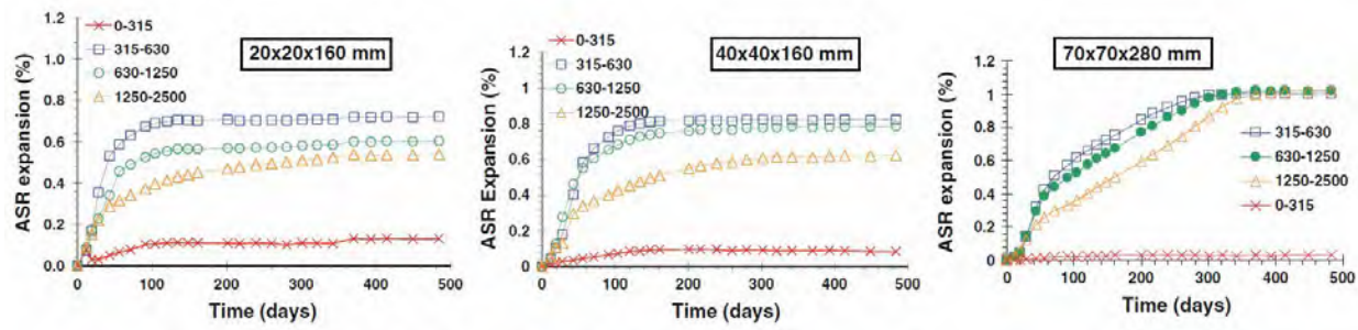
Figure 3.77: ASR expansions on prismatic specimens with siliceous limestone aggregate kept in NaOH solution; Gao et al. (2011)
