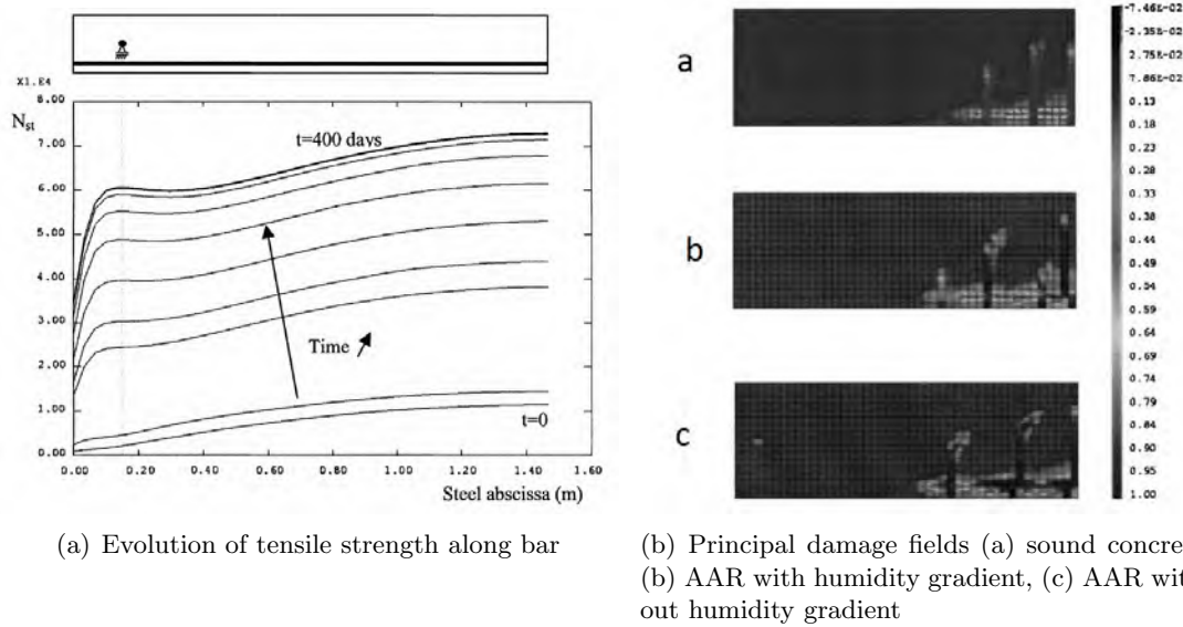
Figure 3.24: Results of numerical simulations by Capra and Sellier (2003)
