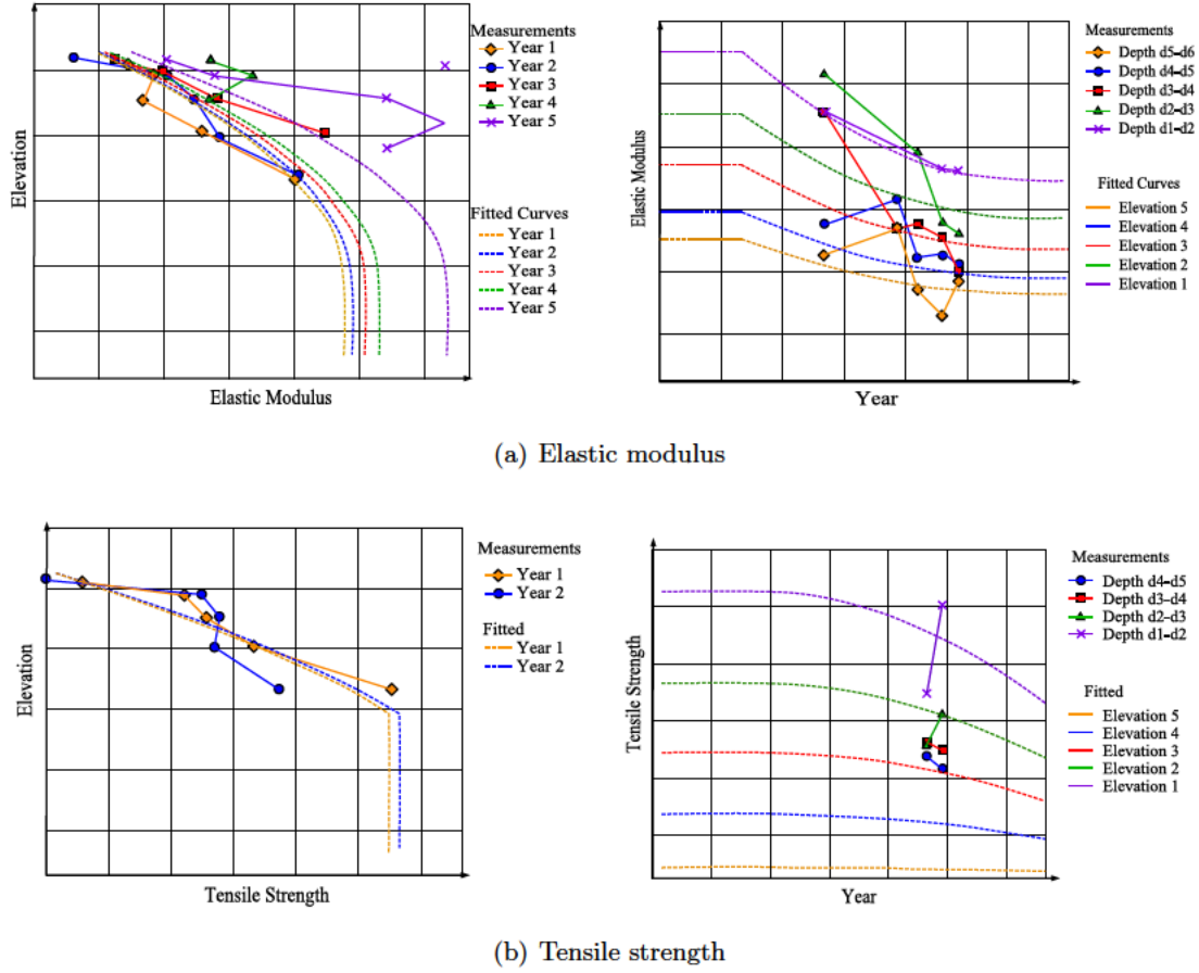
Figure 6.7: Spatial and temporal fitting for concrete mechanical properties based on limited cores and observations (courtesy Y. Gakuhari)
