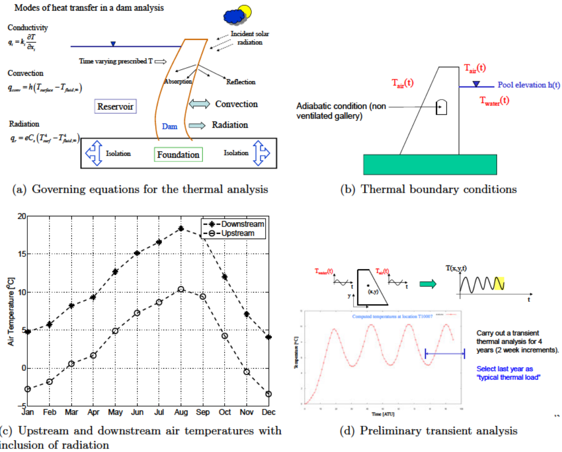
Figure 6.14: Data preparation for thermal analysis of a dam subjected to AAR
