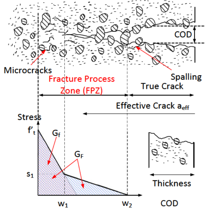
Figure 4.2: Hillerborg's model
