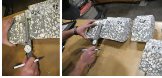
Figure A.8: Measuring specimen dimensions
