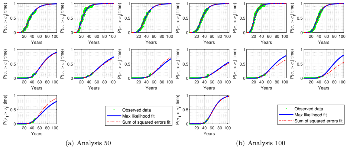
Figure H.7: Probability of Exceedance; Upstream
