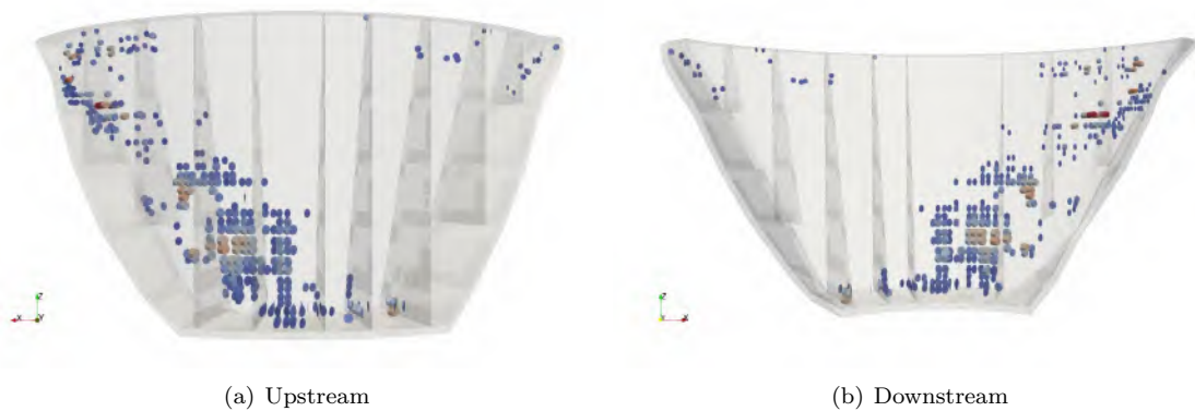
Figure 7.13: Smeared crack profile after 50 years of analysis
