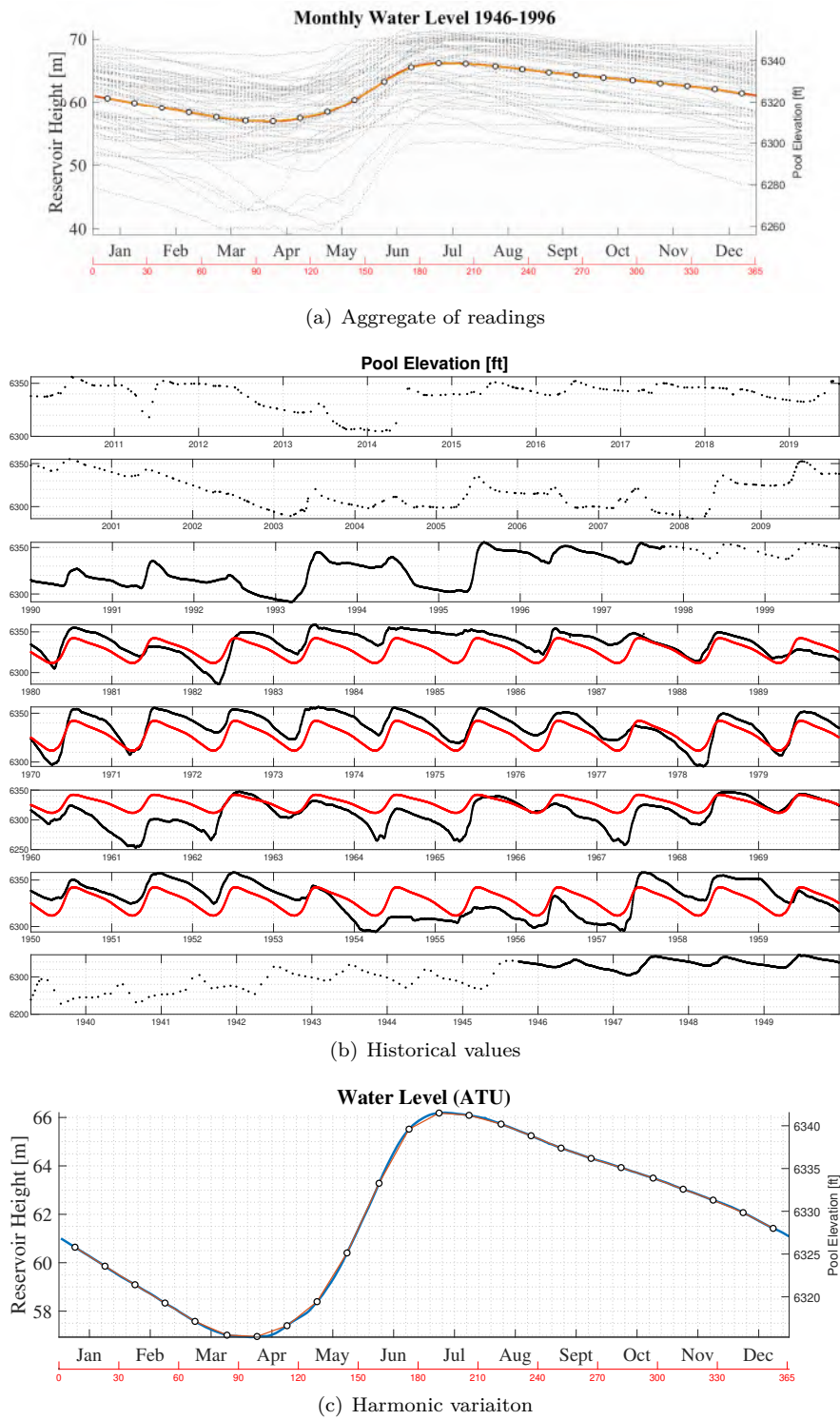
Figure A.27: Recorded pool elevations
