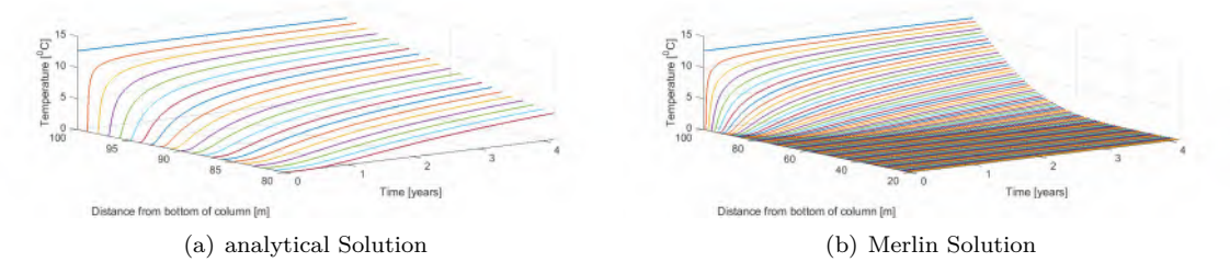
Figure B.11: Thermal analysis results of constant temperature applied at the end of the column
