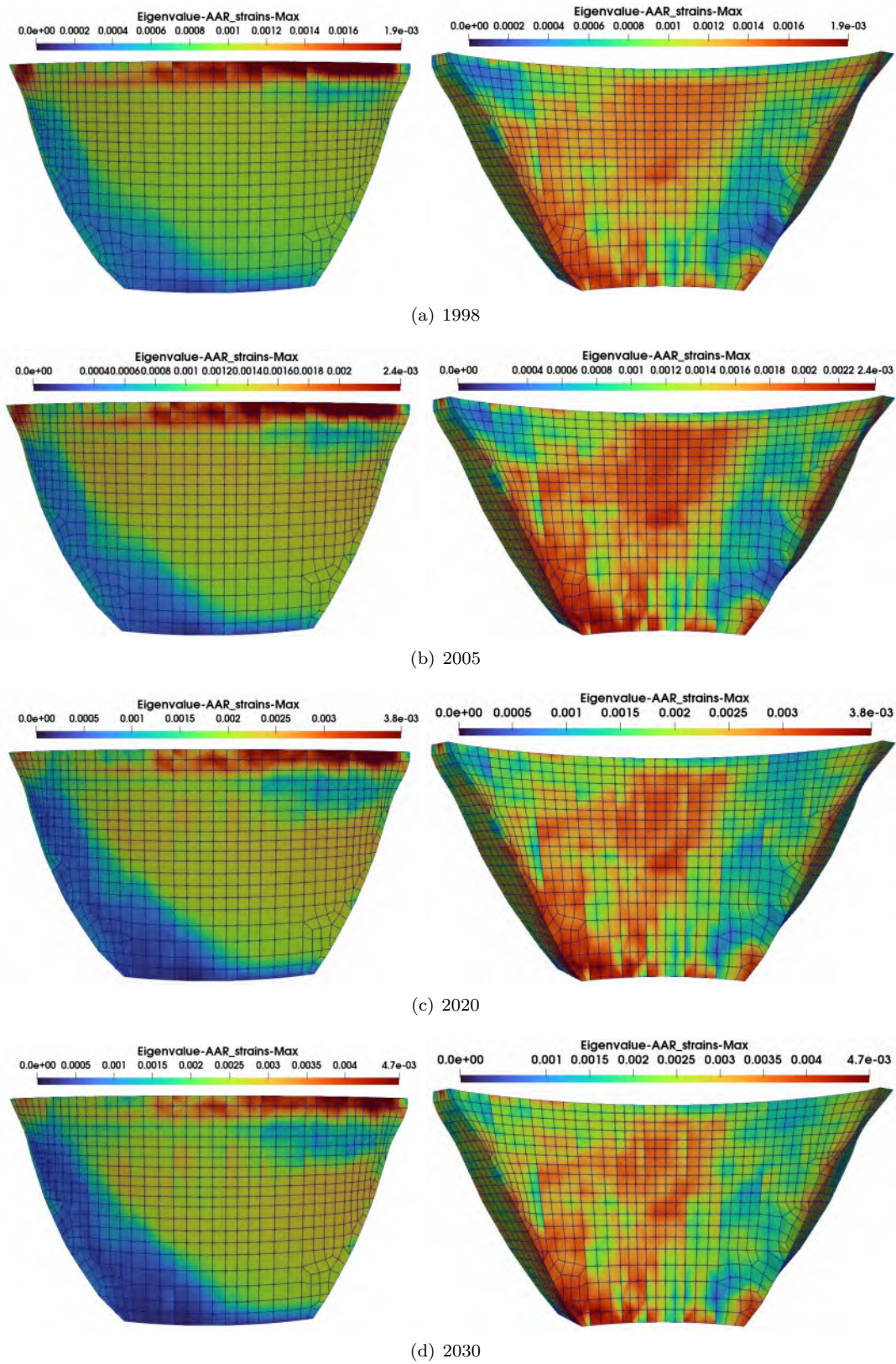
Figure 7.18: AAR development over the time
