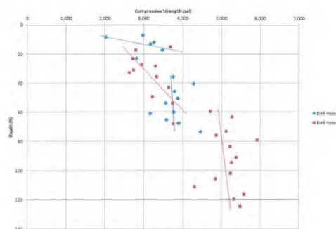
Figure A.9: 2013 Compressive strength data from petrographic study ( usbr-████████-petrography )
