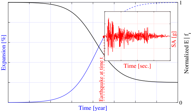
Figure 9.1: Earthquake occurring after substantial AAR expansion
