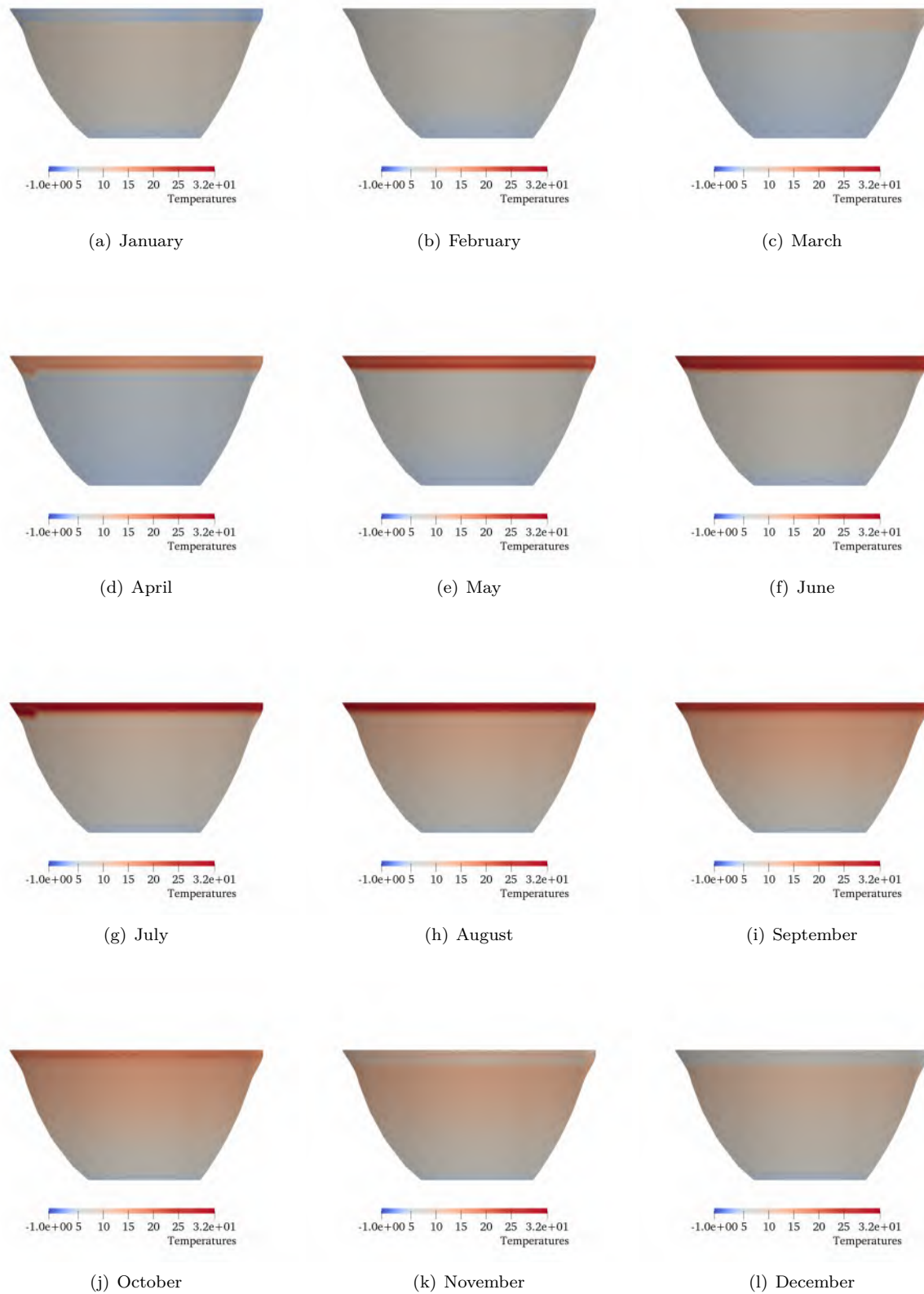
Figure 6.8: Temperature contour plots of various months throughout one year at the upstream face of
