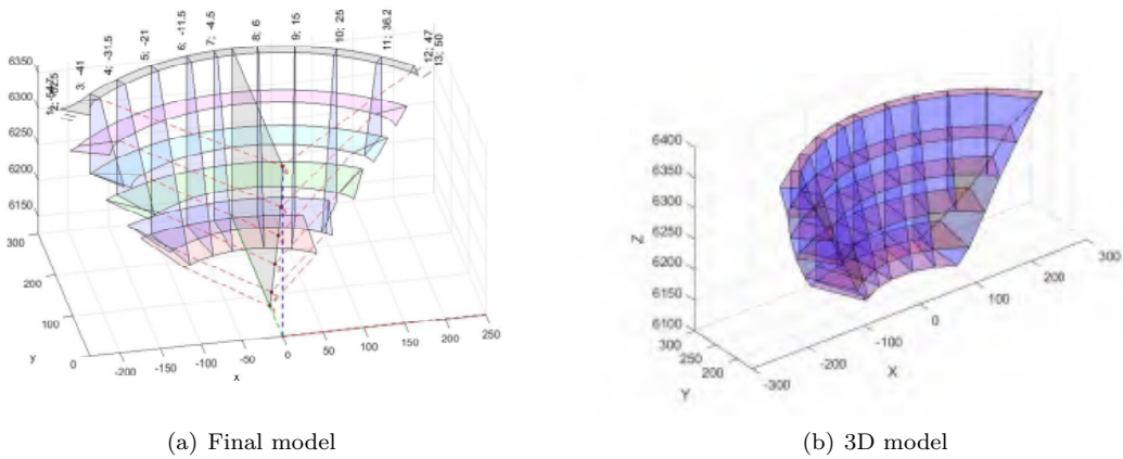
Figure 5.5: Mathematical Modeling of XXXXXXXXXX Dam
