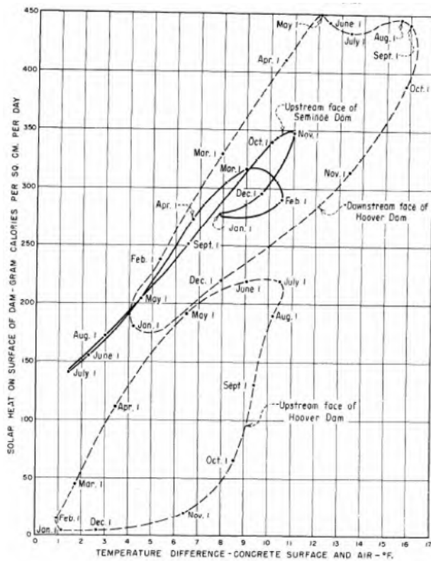
Figure 3.11: Average monthly temperature increase due to solar radiation for upstream face of [REDACTED] from em34empty citation
