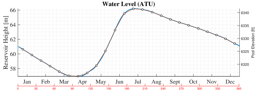
Figure 4.3: Pool Elevations
