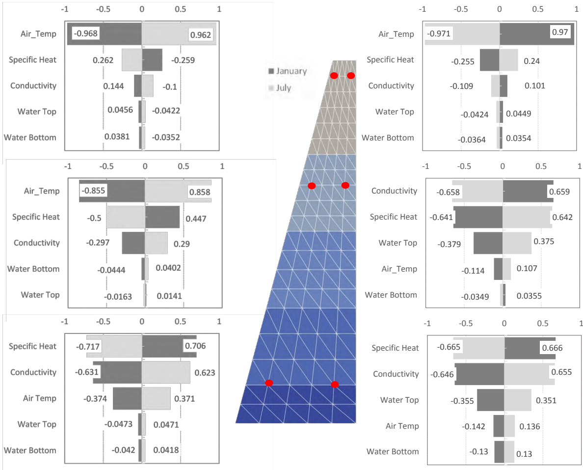
Figure 8.3: Correlation of nodal temperatures and variables at 6 different nodes in January and July
