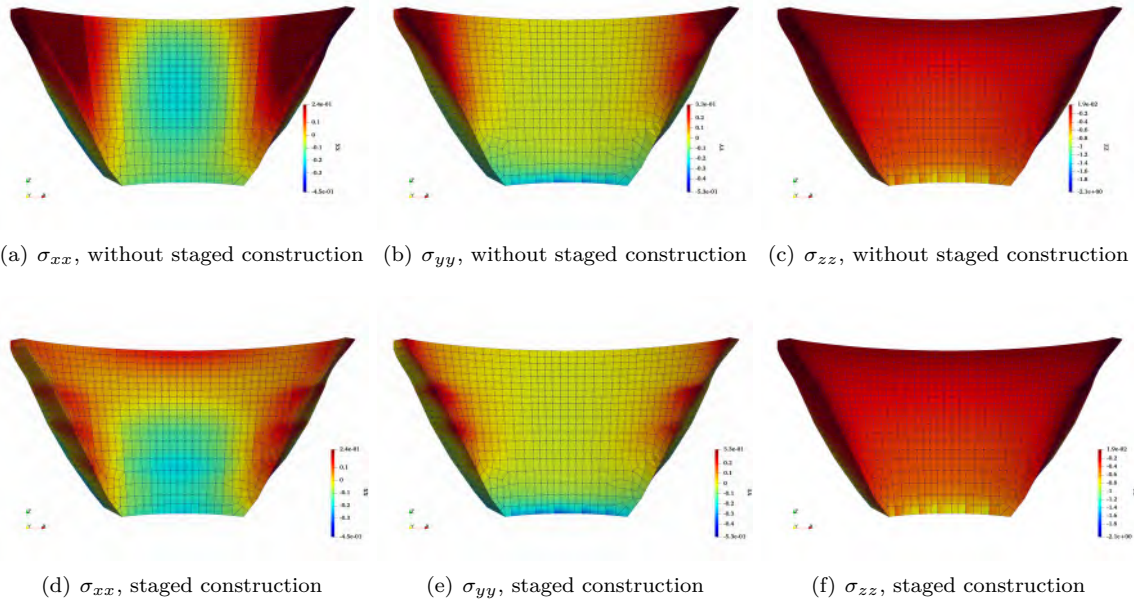
Figure 5.11: Effect of modeling staged construction XXXXXXXXXX Downstream
