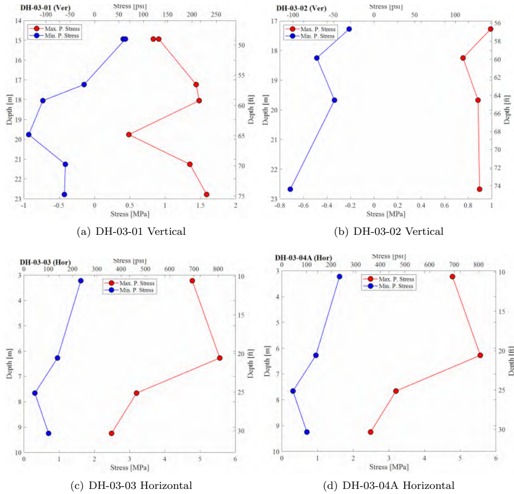
Figure A.16: Results of 2003 overcoring
