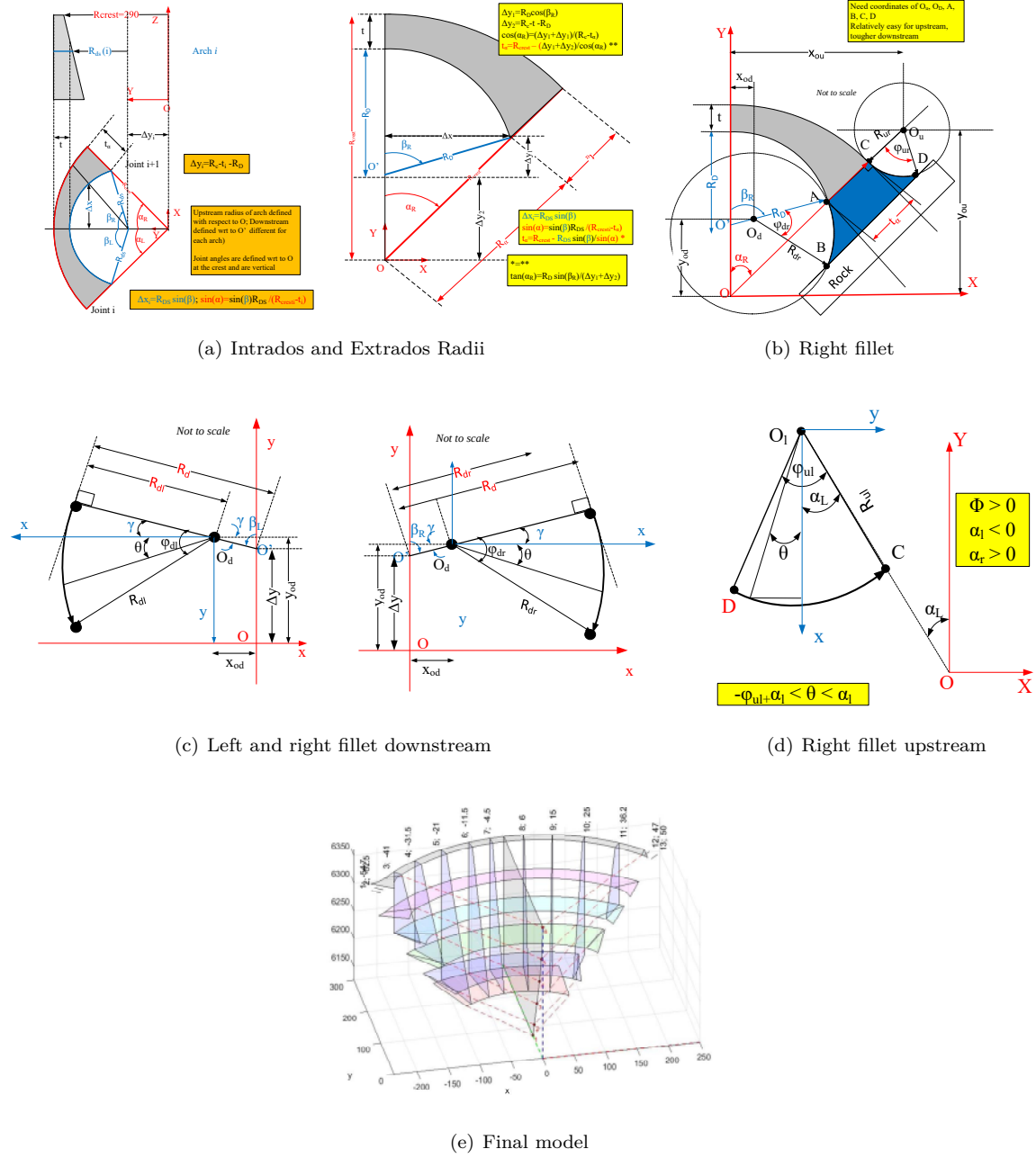
Figure 5.2: Mathematical Modeling of Dam
