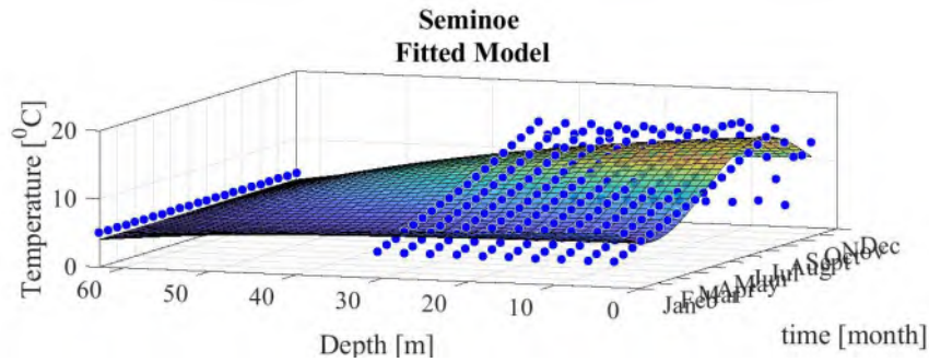
Figure 4.2: [REDACTED] reservoir temperature
