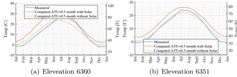
Figure 6.3: Comparison of thermal analysis results with measured values with and without solar radiation
