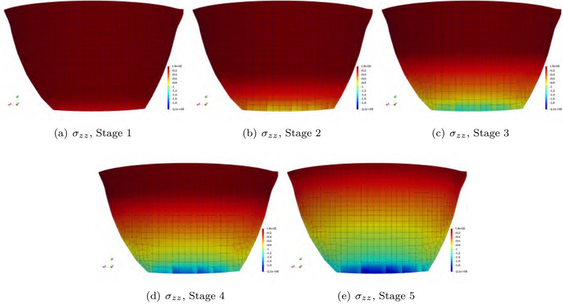
Figure 5.9: Effect of modeling staged construction [REDACTED] Upstream; different stages
