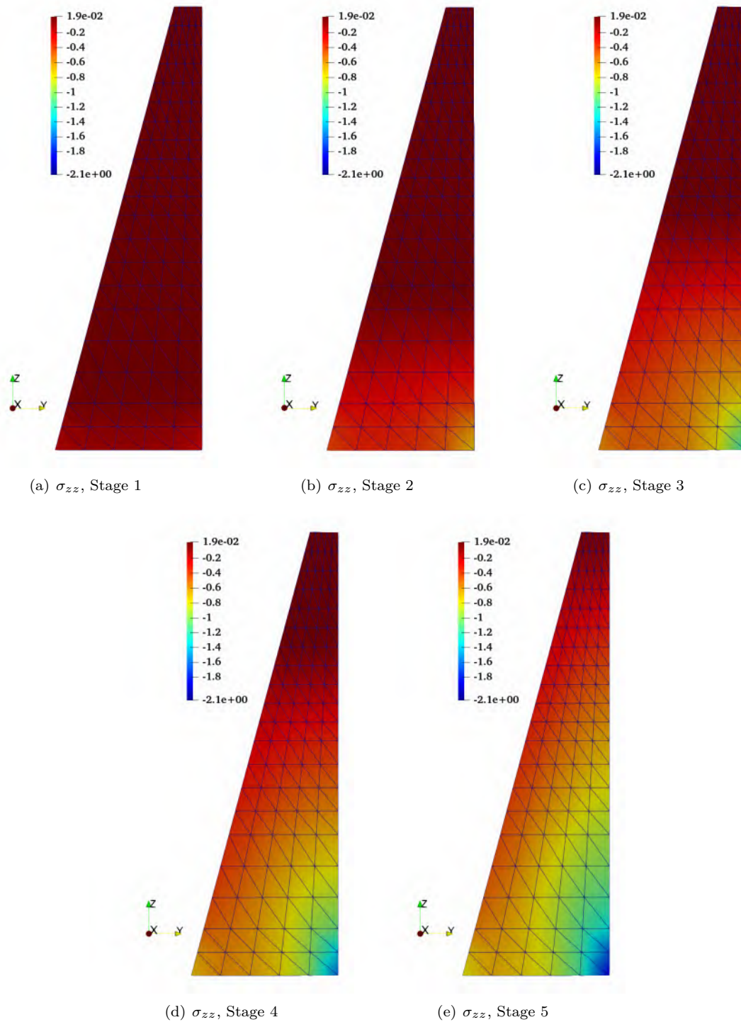
Figure 5.10: Effect of modeling staged construction vertical cut from middle of [REDACTED]; different stages
