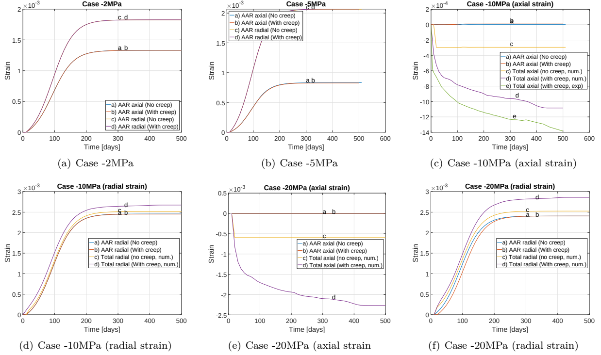
Figure E.5: Numerical results of calibration for Creep, part 2
