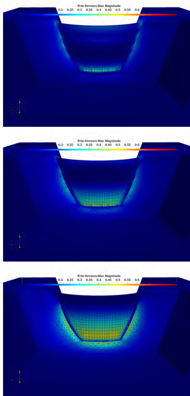
Figure 5.17: Gradual application of hydrostatic load in 3 steps
