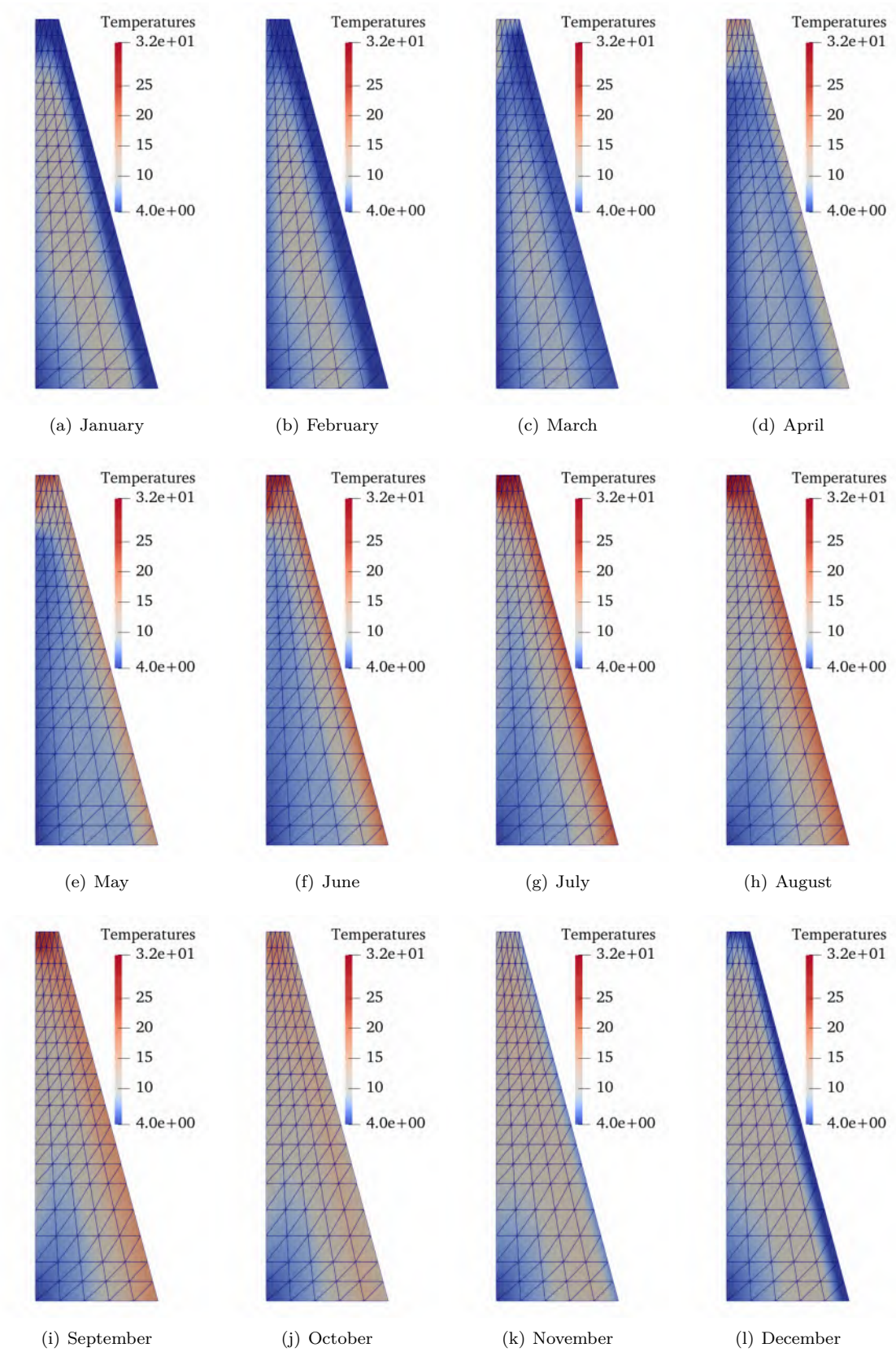
Figure 6.5: Temperature contour plots of various months throughout one year at a vertical section cut from the middle of the arch dam
