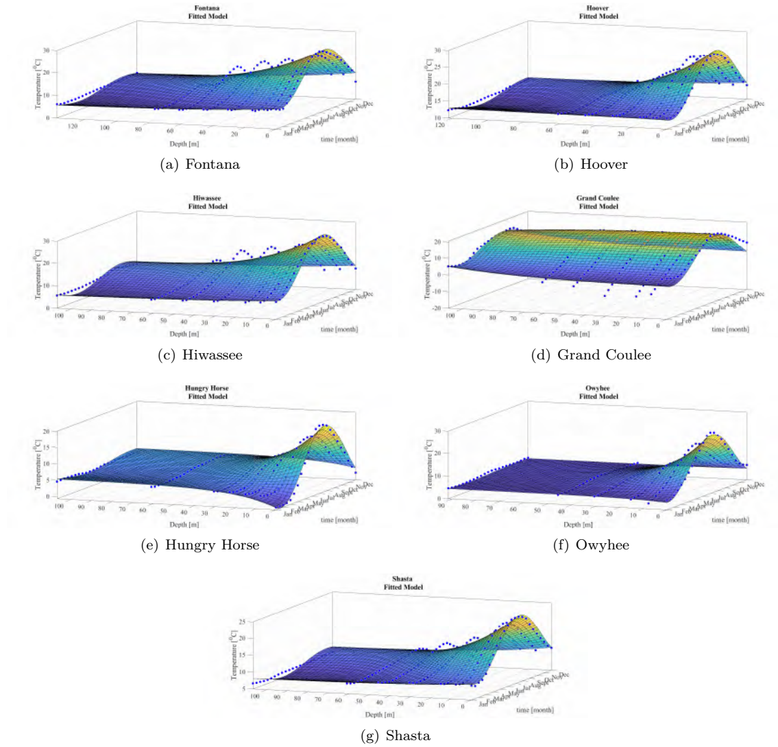
Figure B.6: Fitted dam temperatures from (Model II) Figure B.5
