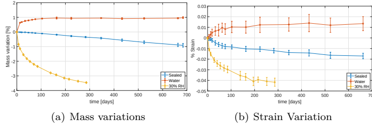
Figure D.3: Non reactive concrete under various RH conditions; ( multon06 )
