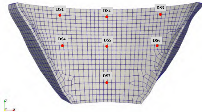
(c) Downstream,Stresses
