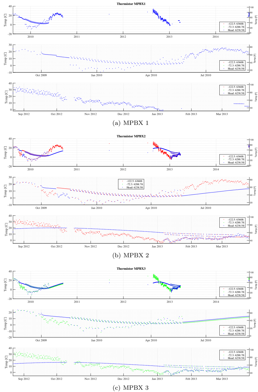
Figure A.18: MPBX Based Concrete temperatures
