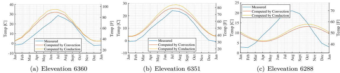
Figure 6.4: Comparison of thermal analysis results with measured values assuming high values for film coefficients
