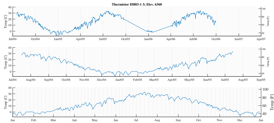
(b) Elevation 6288
