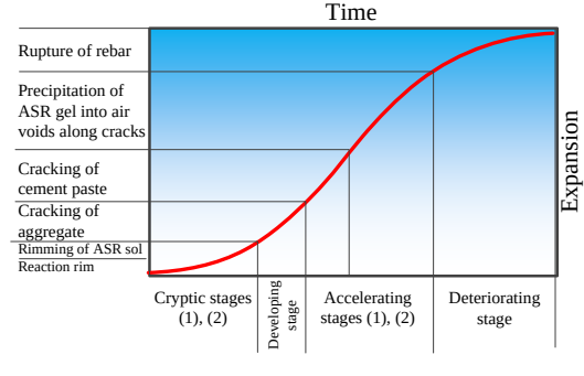
(c) Physical deterioration associated with AAR ( saouma2017riskinformed )
