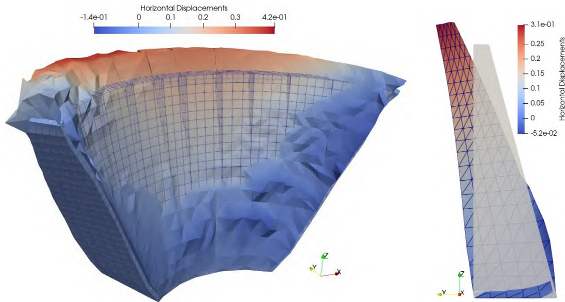
Figure 7.11: Dam deformed shape after 50 years of analysis; Nonlinear analysis
