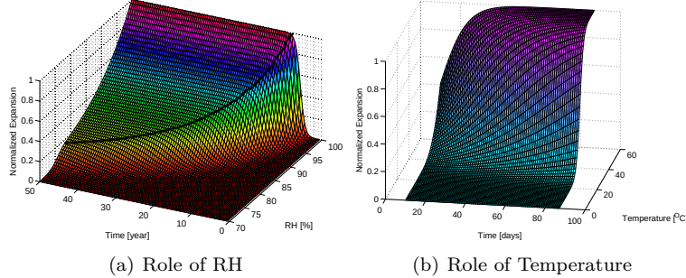
Figure 2.8: Environmental factors affecting AAR expansion
