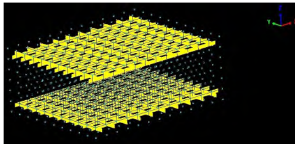
Figure 11.3: 3D finite element model of the reinforcement for panel
