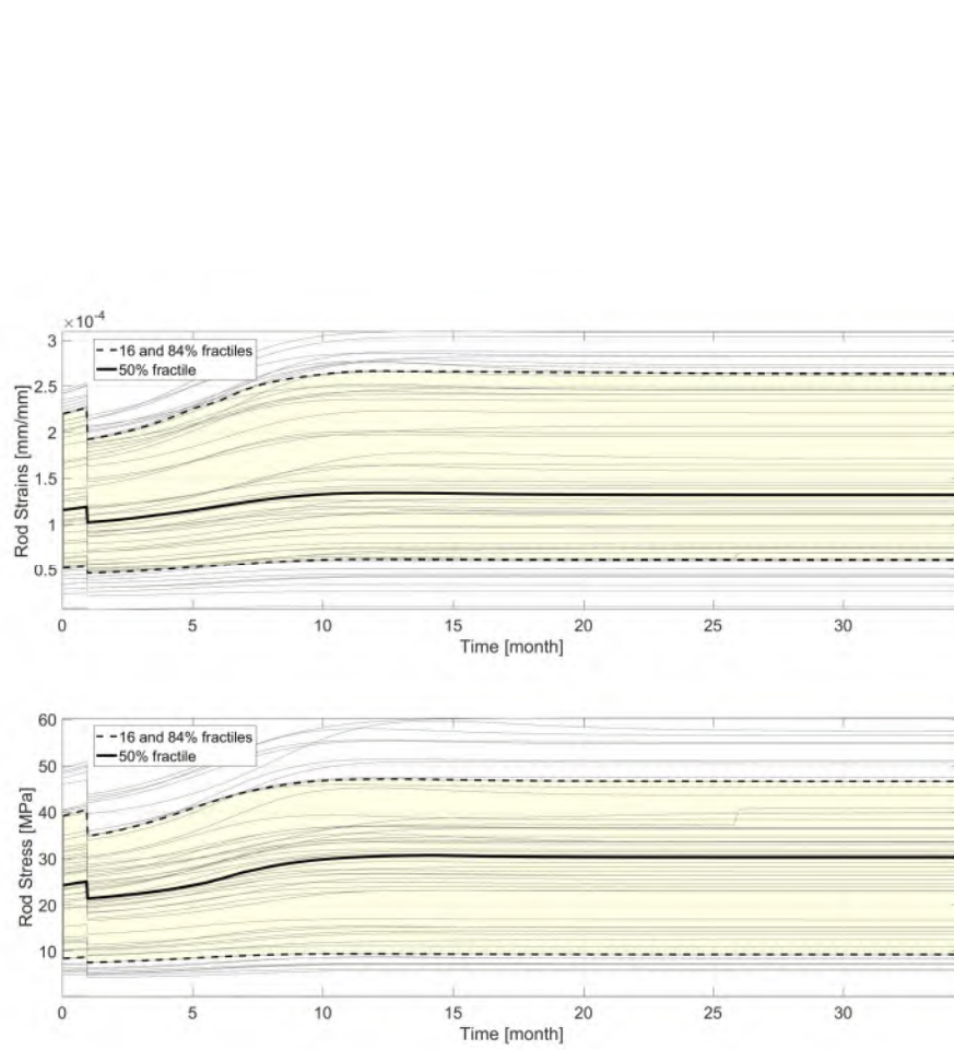
Fig. 3.40. Reinforcement stress and strain at Locator # 8;<2.14, 1.886, 0.8827>
