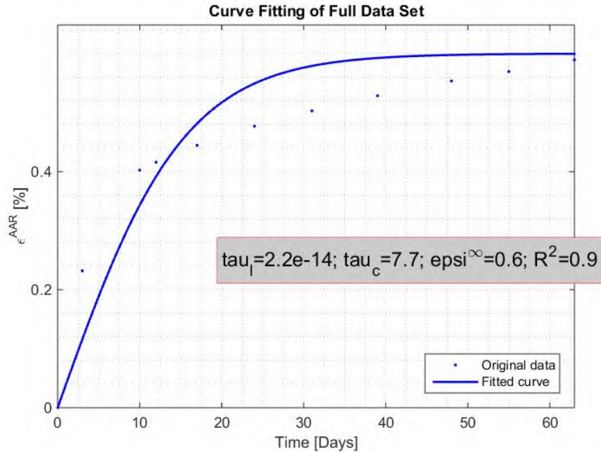
Figure 87 - Curve fitting data from concrete mix 5 (80C, 1M NaOH) to Larive's kinetic model.
