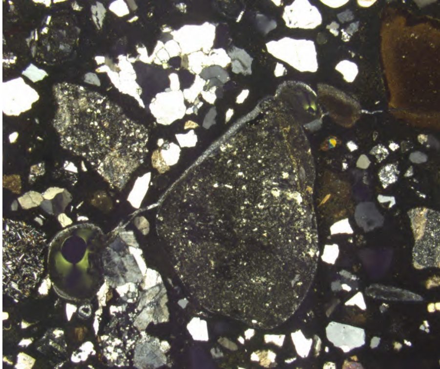
Figure 48 - Mortar-bar with crushed coarse aggregate – same area as in Figure 46 and Figure 47. Cross polarized light. Magnification: x25
