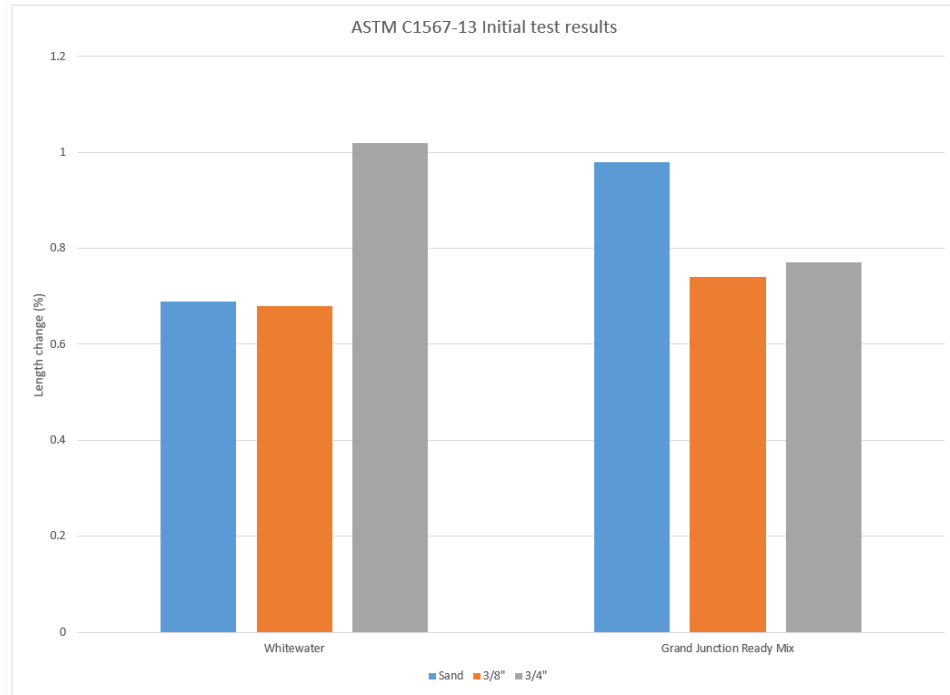
Figure 20- Summary of 16-day ASTM C1567 results
