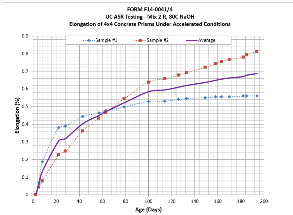
Figure 79 - Elongation of Mix 2 Reactive, accelerated conditions
