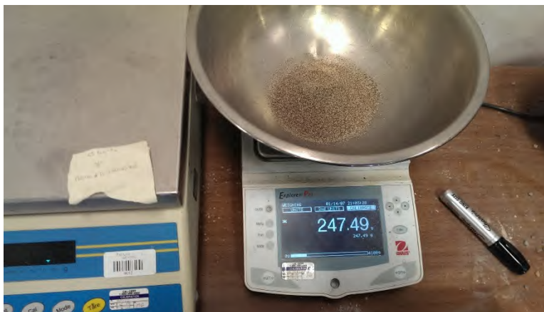
Figure 10 - Balance used to weigh dried aggregate
