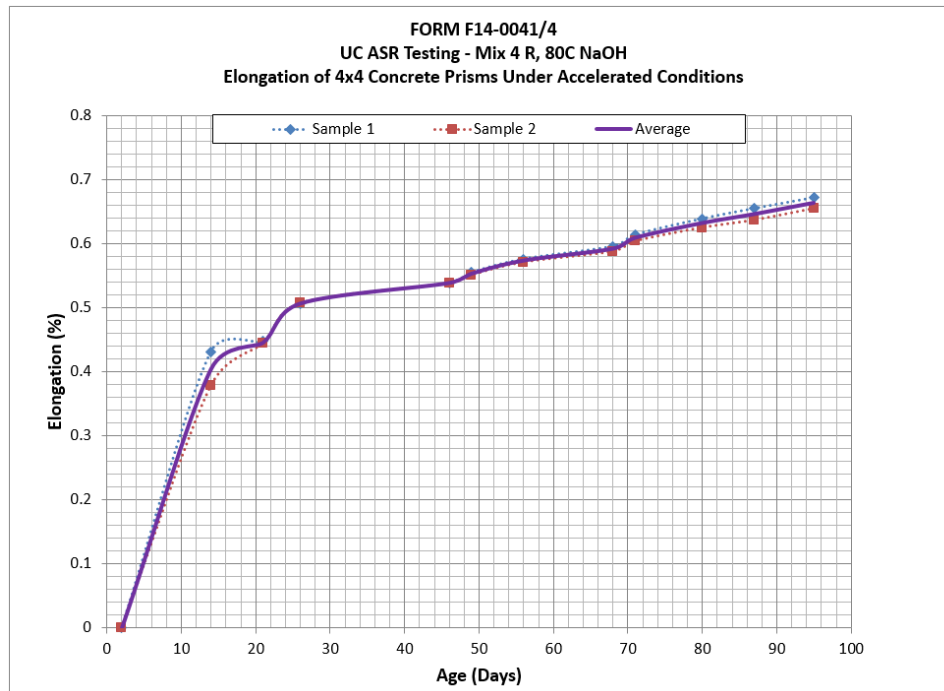
Figure 84 - Elongation of Mix 4, Reactive under accelerated conditions
