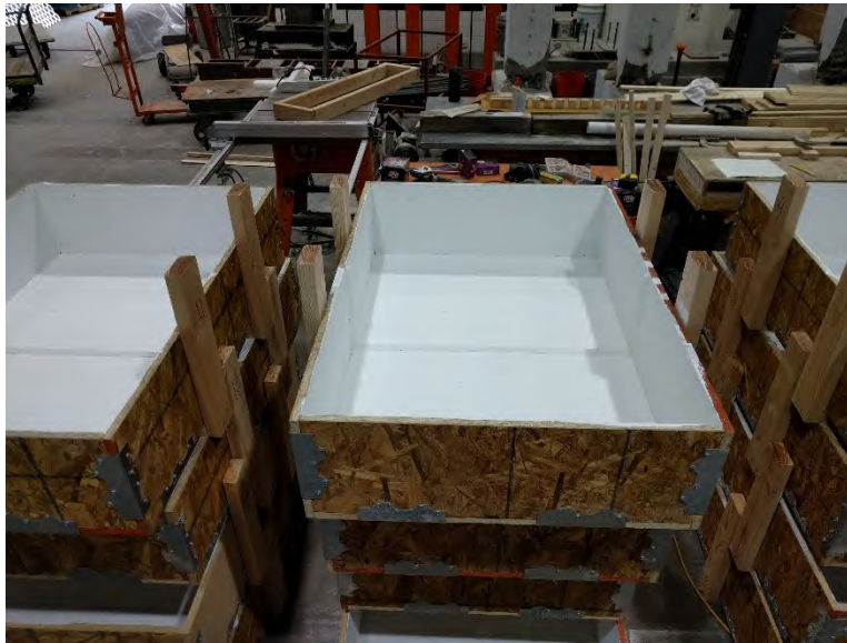
Figure 105 - Assembled and painted formwork. Seventeen forms were built in total.
