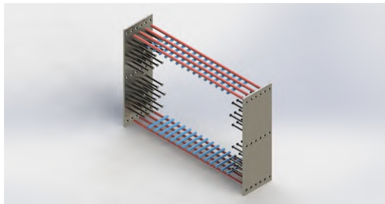
Figure 95 - Shear specimen with concrete hidden. Red bars correspond to axial reinforcement and resist shear by dowel action. Blue bars correspond to the azimuthal reinforcement and are not engaged in shear.
