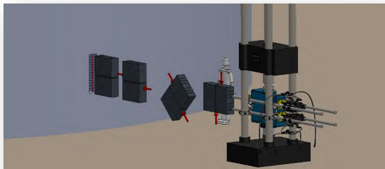
Figure 91 - Specimens are rotated 180 degrees about azimuthal direction
