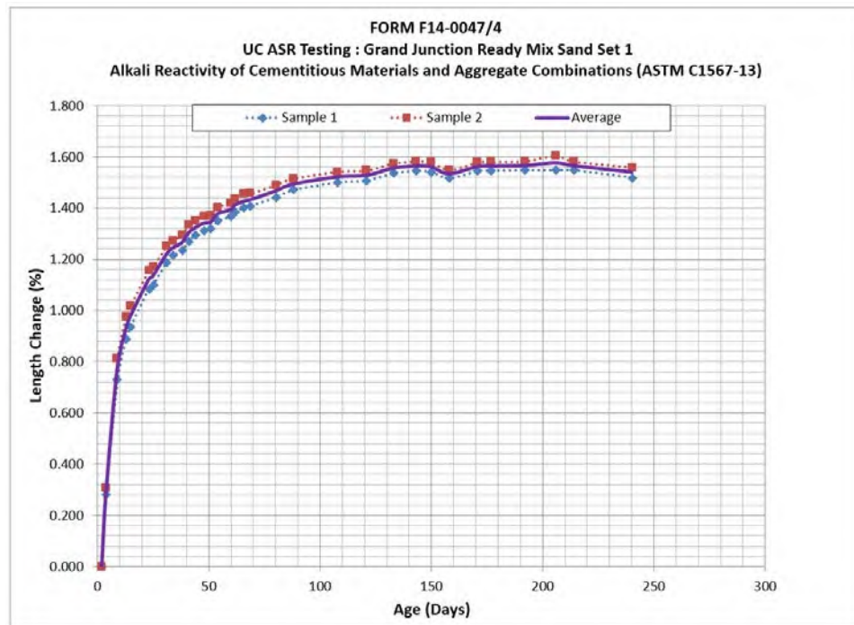
Figure 24 - Mortar bar expansion vs. time, Grand Junction Ready Mix sand
