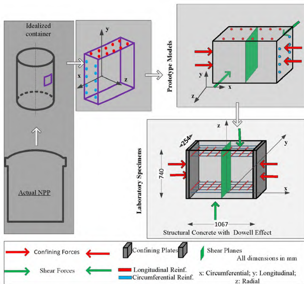
Figure 93 Specimen internal reinforcement and applied forces
