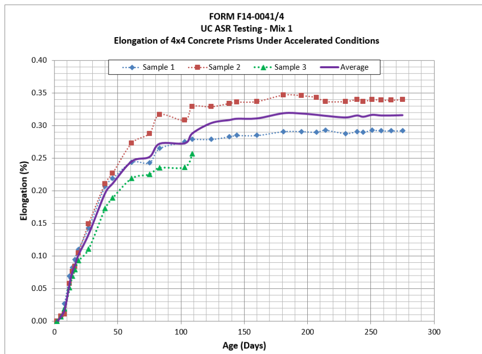
Figure 77 - ASR expansion of Mix 1
