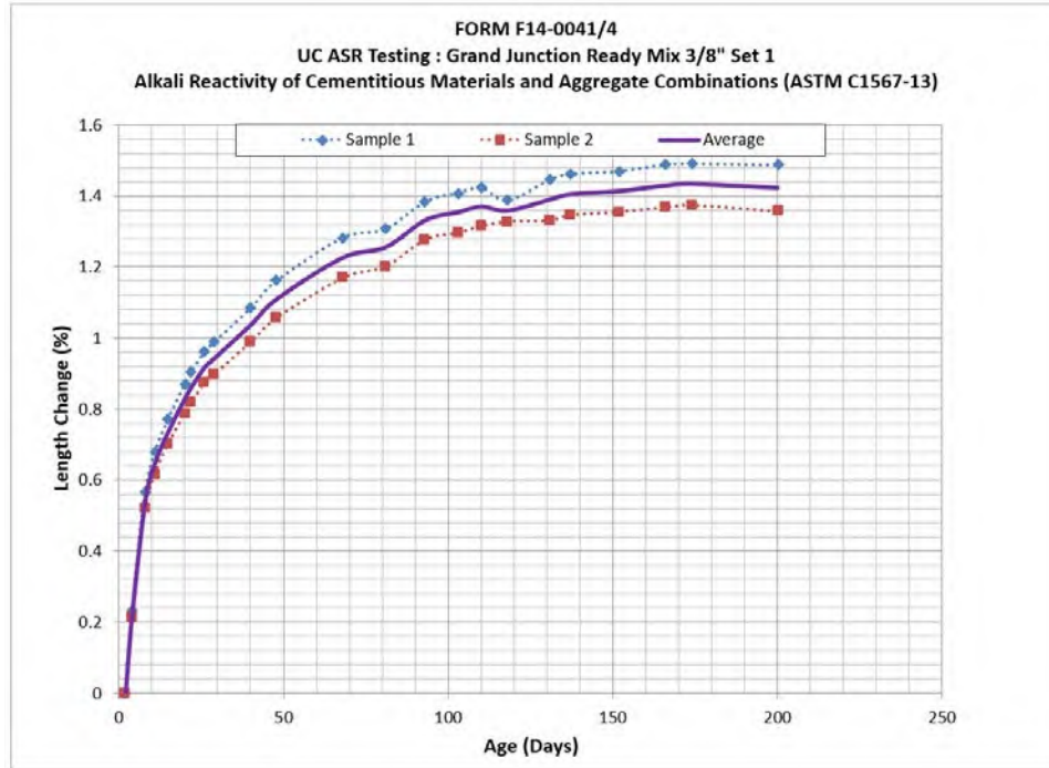
Figure 25 - Mortar bar expansion vs. time, Grand Junction Ready Mix 3/8" aggregate
