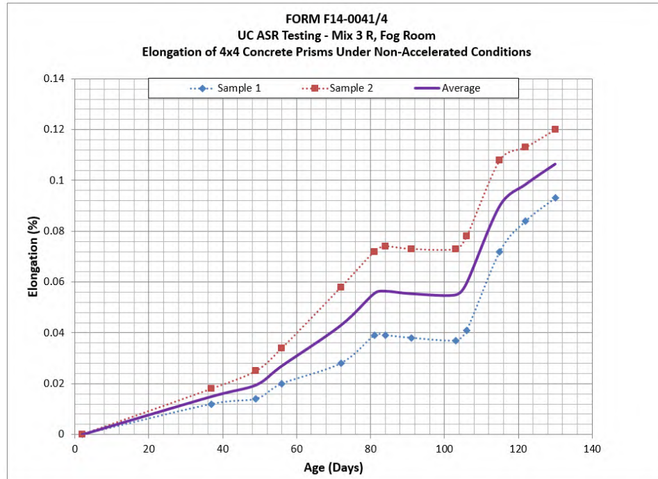
Figure 81 - Elongation of Mix 3, Reactive, under nonaccelerated conditions
