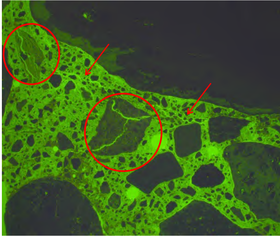
Figure 43 - Concrete sample. Fluorescent light. Magnification: x12.5
