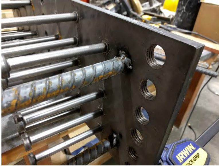
Figure 103 - MIG-welded joint between #6 rebar and sample end plates.
