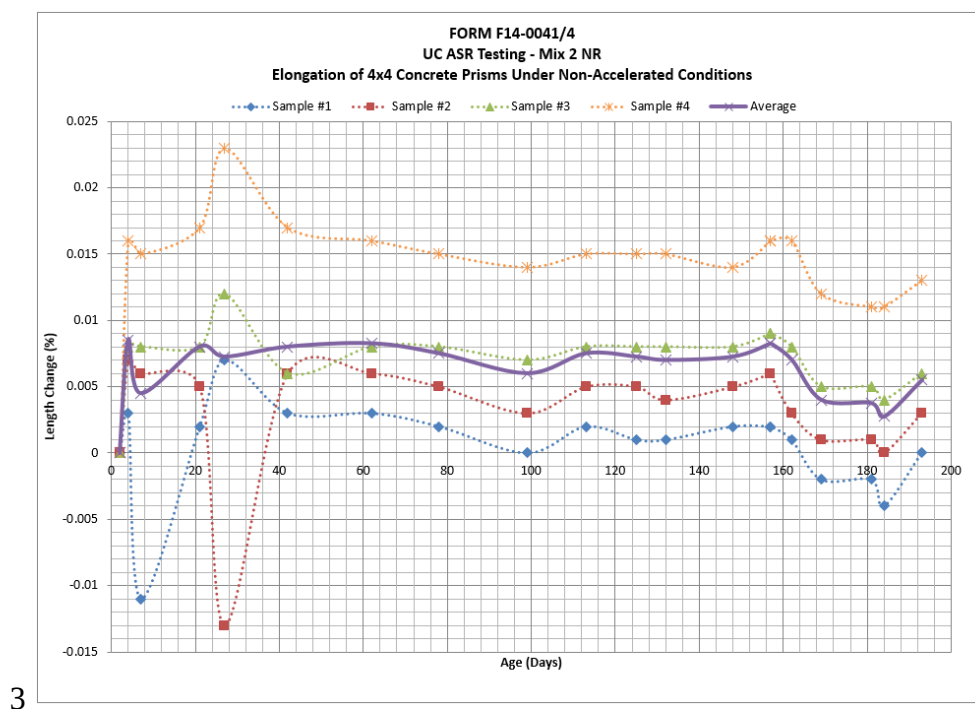
Figure 80 - Elongation of Mix 2 Nonreactive, non-accelerated conditions
