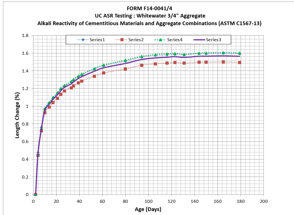
Figure 23 - Mortar bar expansion vs. time, Whitewater 3/4" aggregate
