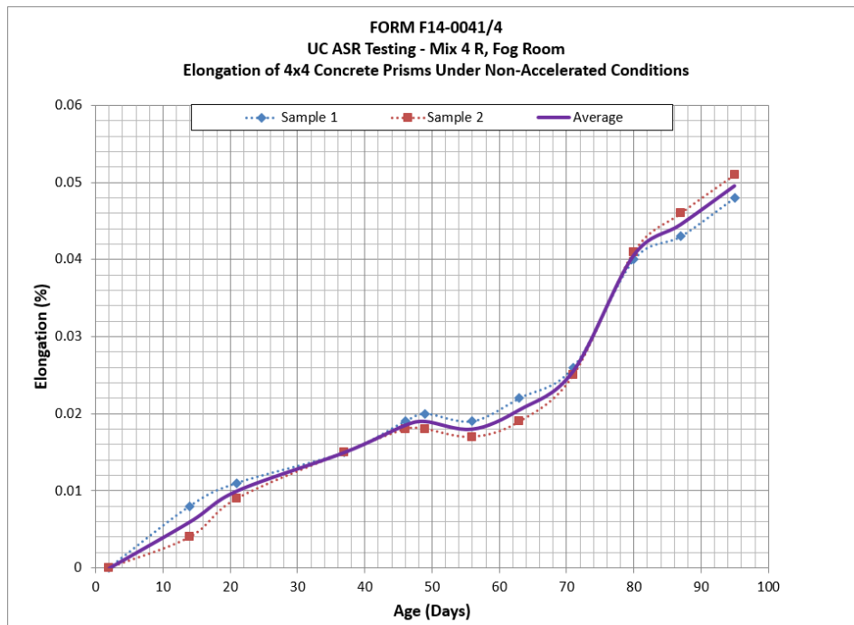
Figure 83 - Elongation of Mix 4, Reactive, under nonaccelerated conditions. Note the dip between 50 days and 70 days. During this time period only one of three Hydrofogger units were operational.
