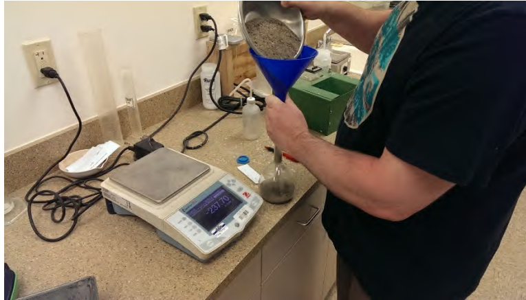
Figure 36 - Adding fine aggregate to volumetric flask.
