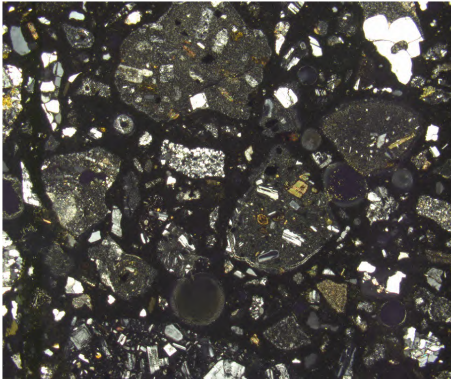
Figure 51 - Mortar-bar with fine aggregate – the same area as in Figure 49 and Figure 50. Cross polarized light. Magnification: x25
