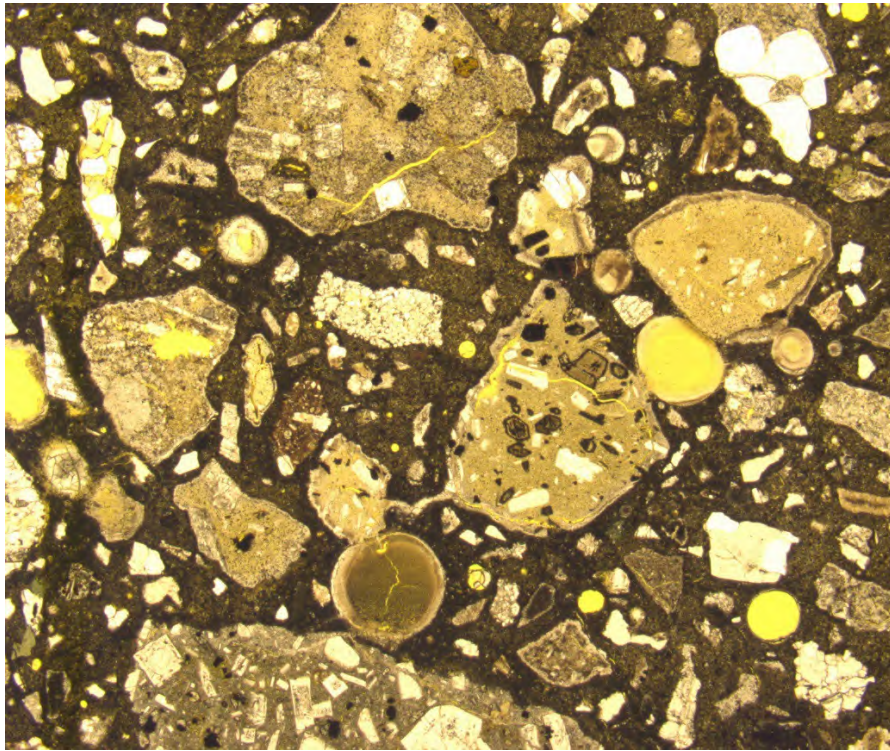
Figure 50 - Mortar-bar with fine aggregate – the same area as in Figure 49. Plane polarized light. Magnification: x25
