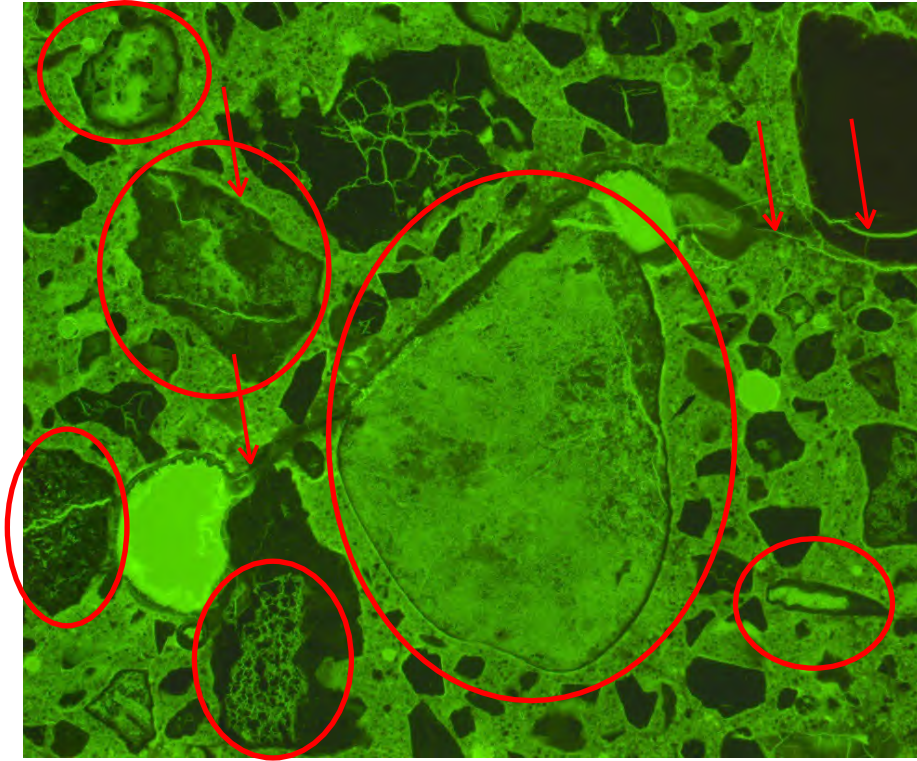
Figure 46 - Mortar-bar with crushed coarse aggregate: Fluorescent light. Magnification: x25
