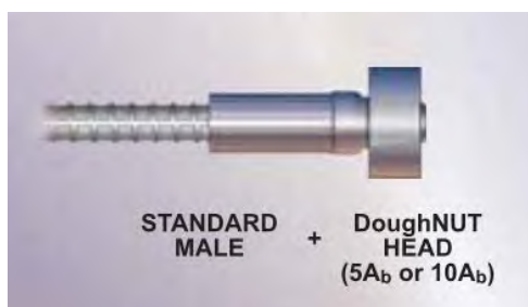
Figure 96 - A threaded 'DoughNUT' connection manufactured by BarSplice Products of Dayton, OH. This is one of the options considered for terminating rebar. Unfortunately, it is too large to fit in the narrow shear sample.
