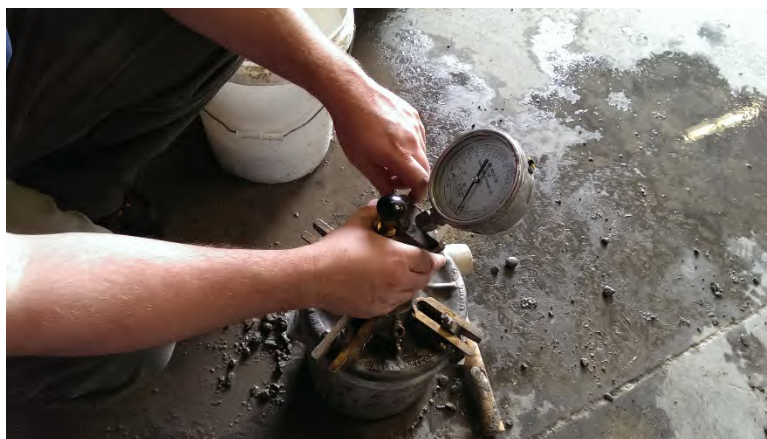
Figure 63 - The top portion of the air meter is installed.
