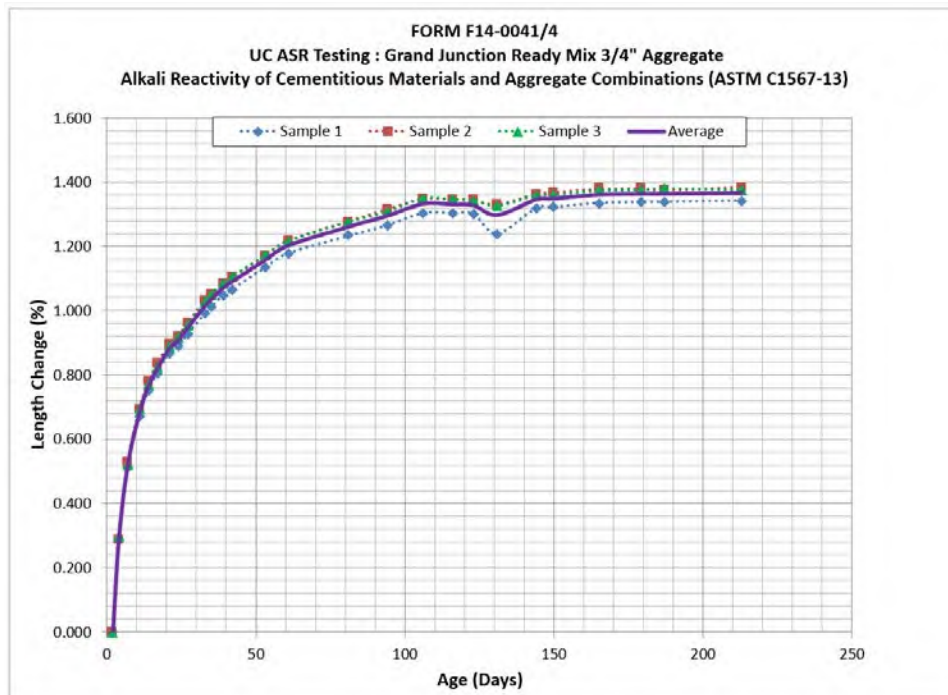
Figure 26 - Mortar bar expansion vs. time, Grand Junction 3/4" aggregate
