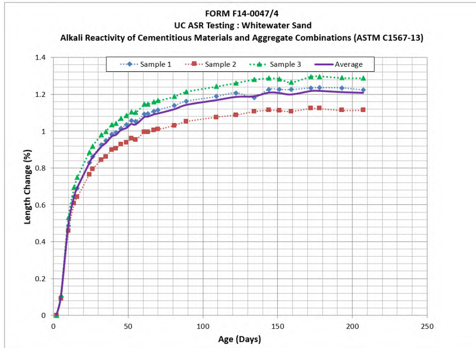
Figure 21 - Mortar bar expansion vs. time, Whitewater sand
