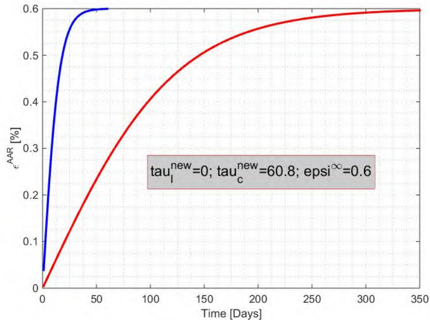
Figure 88 - Expansion vs time for 80C (blue line) and 38C (red line)
