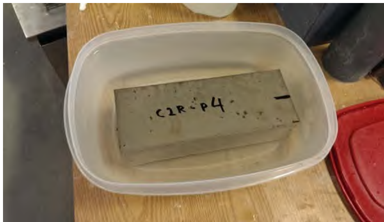
Figure 75 - Concrete prism in container with 1N NaOH.
