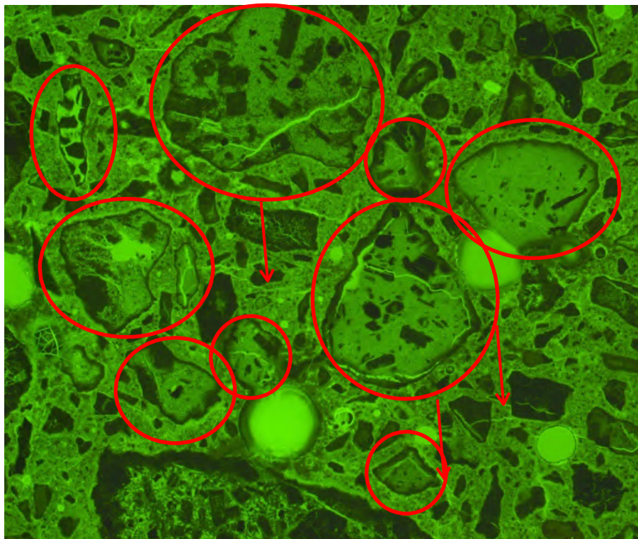
Figure 49 - Mortar-bar with fine aggregate. Fluorescent light. Magnification: x25
