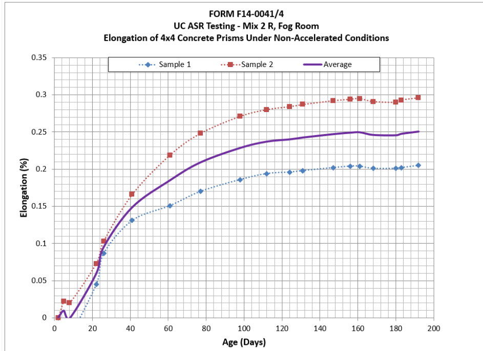
Figure 78 - Elongation of Mix 2 Reactive, non-accelerated conditions
