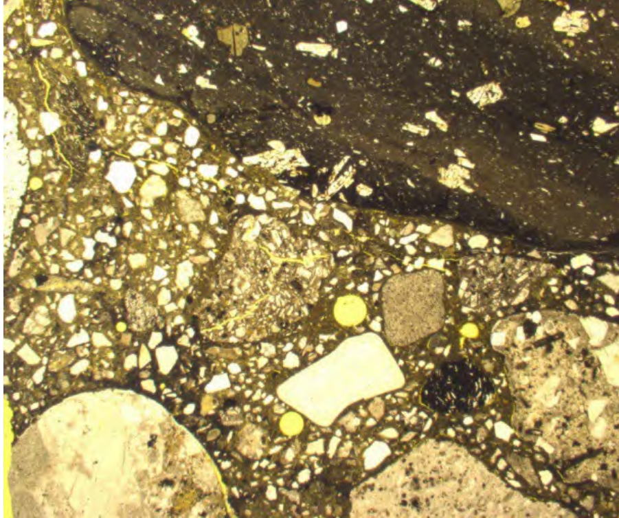
Figure 44 - Concrete sample - the same area as in Figure 43. Plane polarized light. Magnification: x12.5
