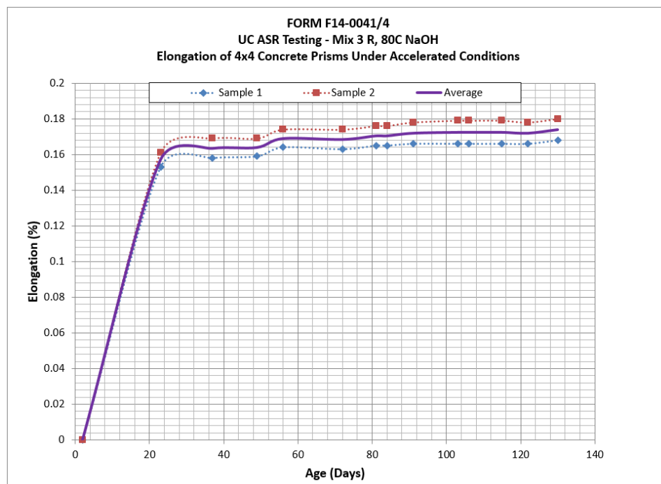
Figure 82-Elongation of Mix 3, Reactive under accelerated conditions
