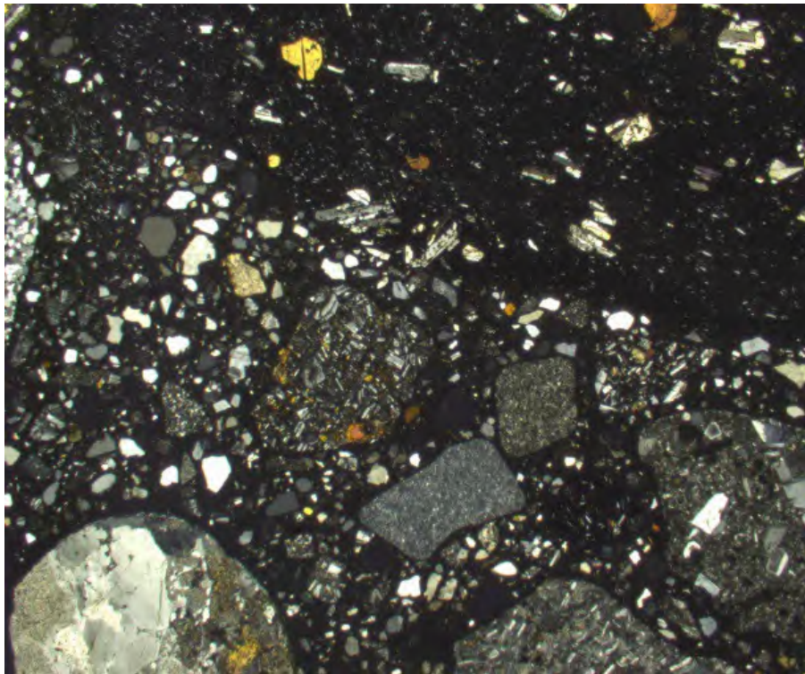
Figure 45 - Concrete sample – the same area as in Figure 43 and Figure 44. Cross polarized light. Magnification: x12.5.
