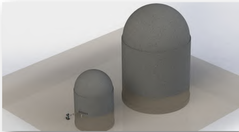
Figure 89 - Prototype system (right) with model system (left)
