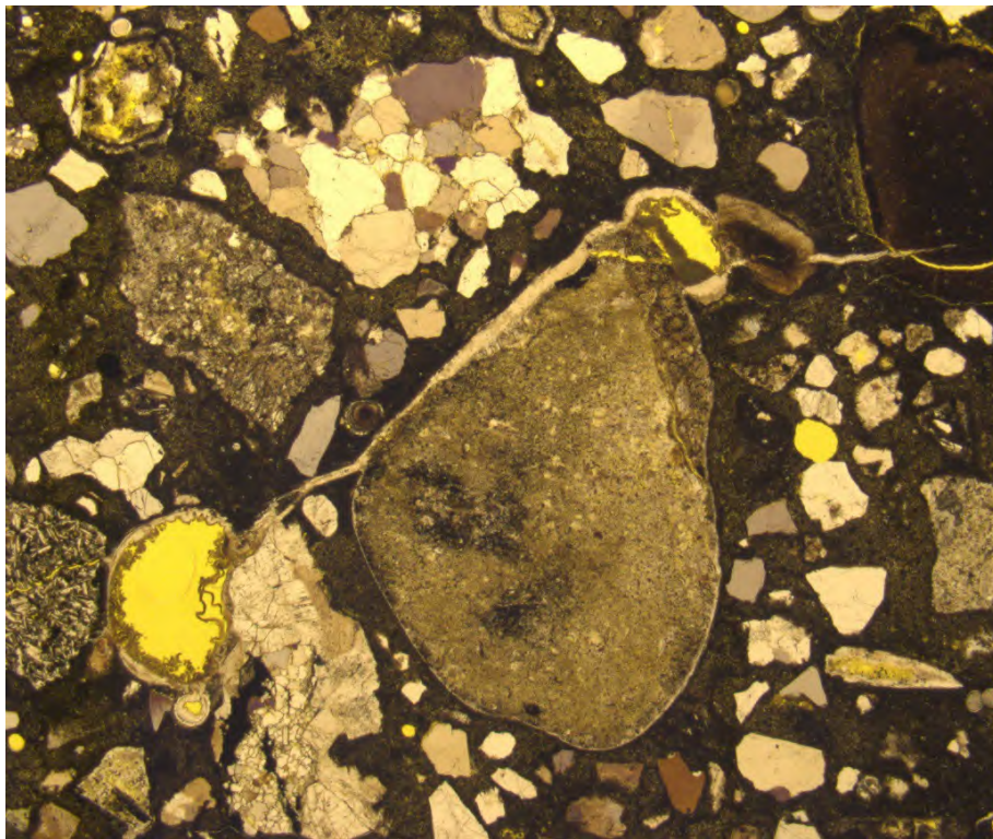
Figure 47 - Mortar-bar with crushed coarse aggregate – the same area as in Figure 46. Plane polarized light. Magnification: x25.
