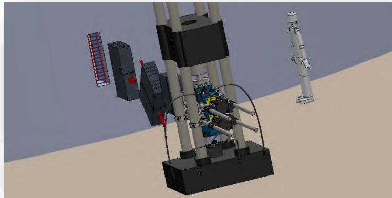
Figure 92 - Rebar in model system is oriented in the axial (red) and azimuthal (blue) directions
