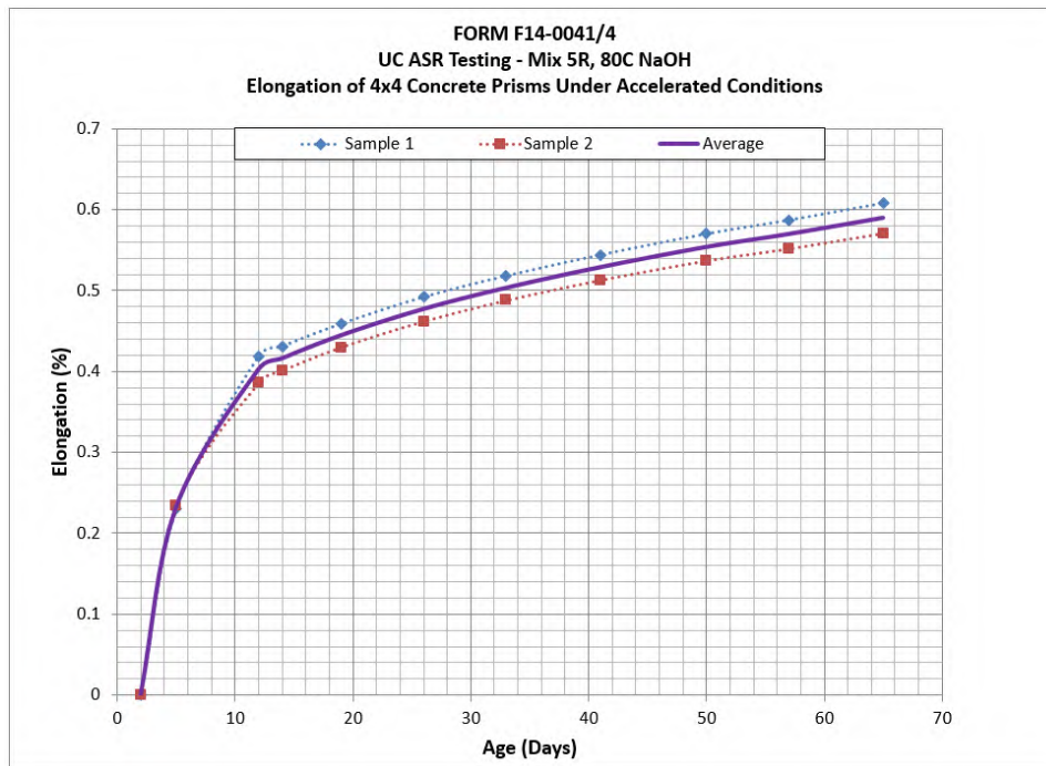
Figure 86 - Elongation of Mix 5, Reactive under accelerated conditions
