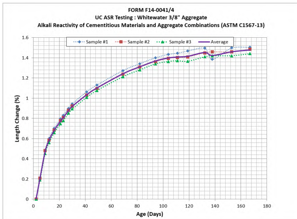
Figure 22 - Mortar bar expansion vs. time, Whitewater 3/8" aggregate
