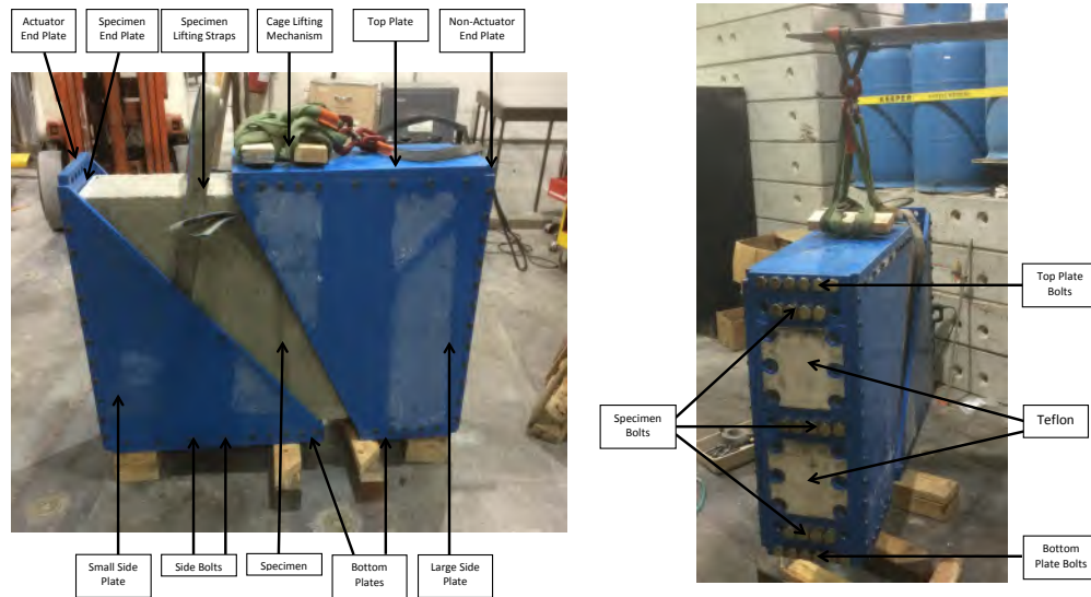
Figure 3.1: Specimen description
