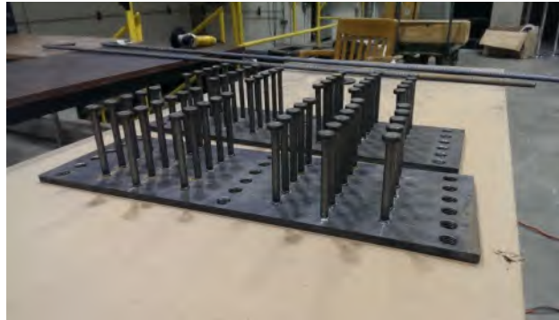
(c) Internal specimen reinforcement
