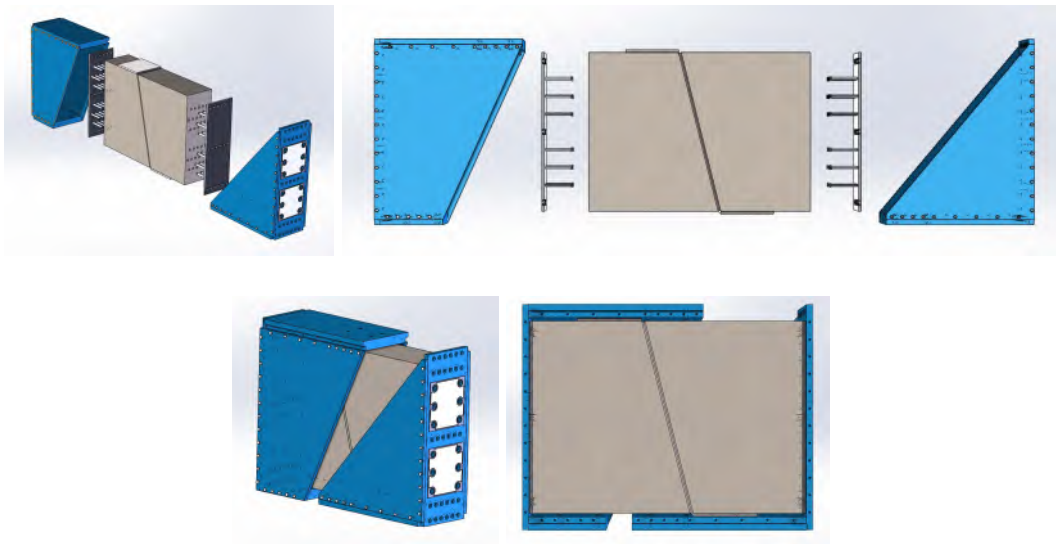
Figure 1.3: Specimen details
