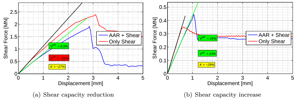
Figure 16: Impact of ASR on shear capacity of concrete panels from a NPP (Saouma et al., 2016)
