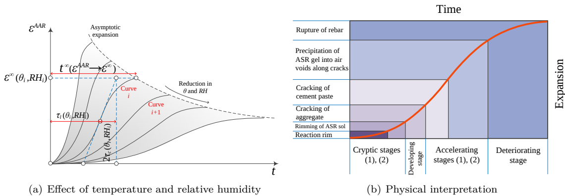
Figure 18: AAR expansion curve Saouma et al., 2015
