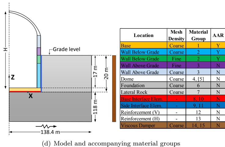
Figure 15: Geometry and model idealization
