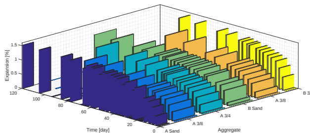
Figure 1: Expansion of mortar bar tests
