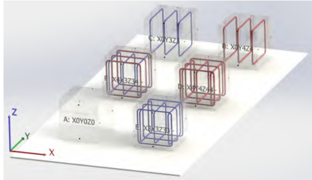
Figure 2: 14" \times 14" \times 14" blocks with various reinforcements
