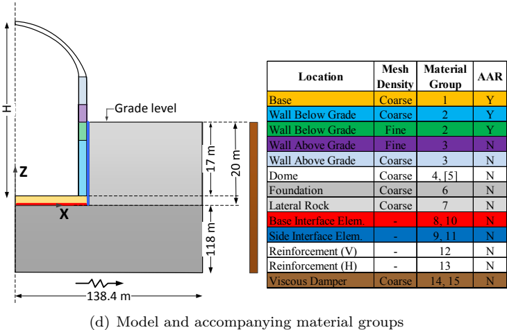
Figure 15: Geometry and model idealization
